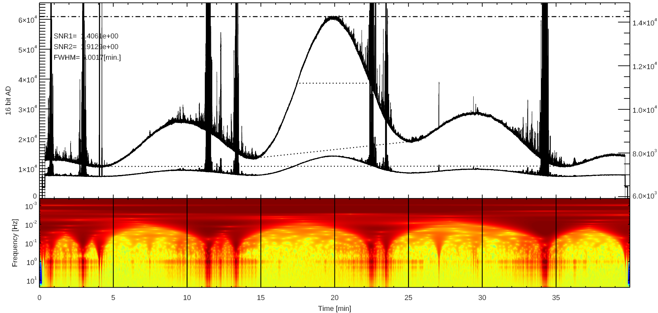
C 3C144 (/home4/archive/swift/dat/2025/10/T20251029023718.dat)
