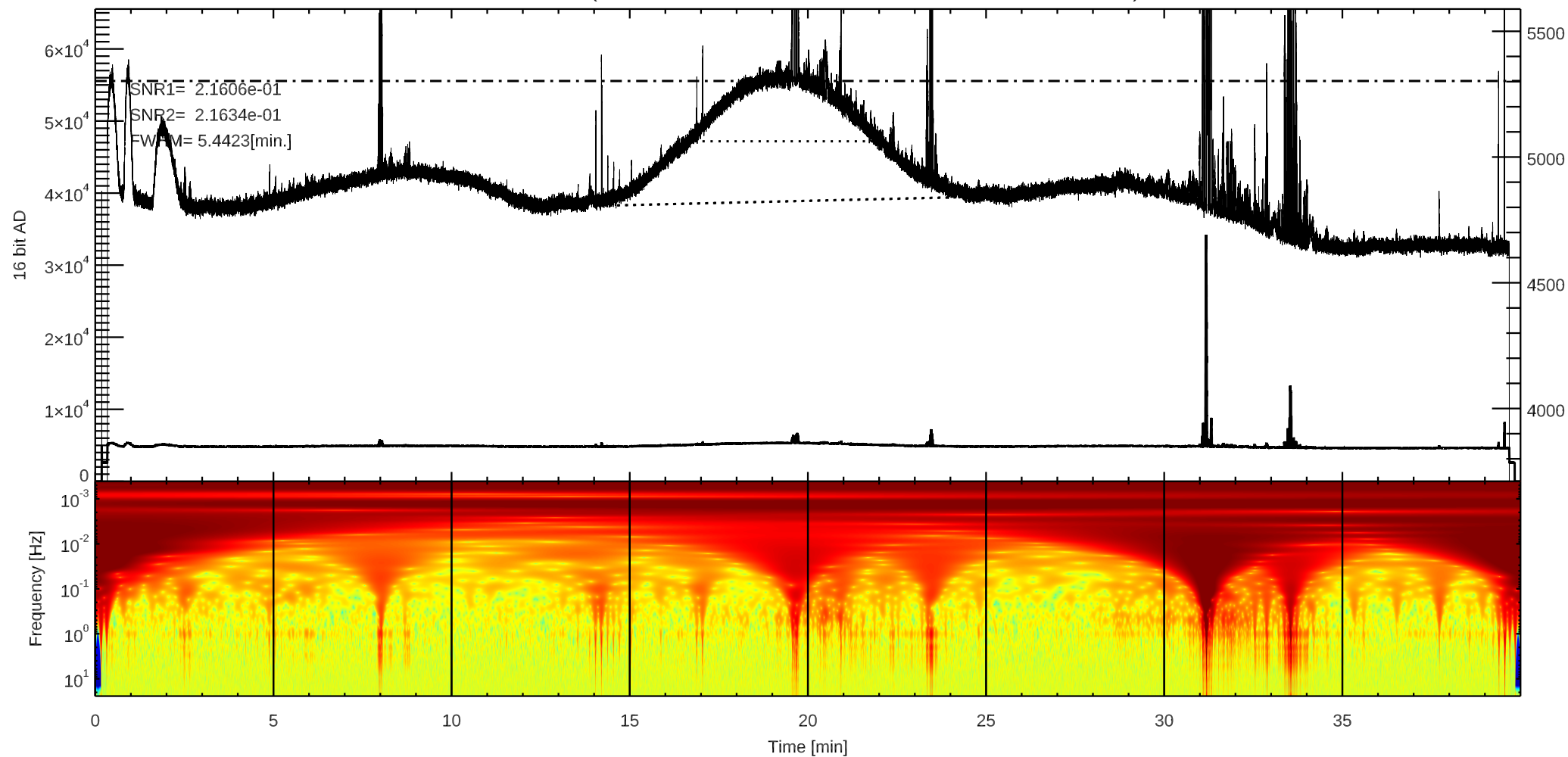
C 3C157 (/home4/archive/swift/dat/2025/10/T20251004045900.dat)
