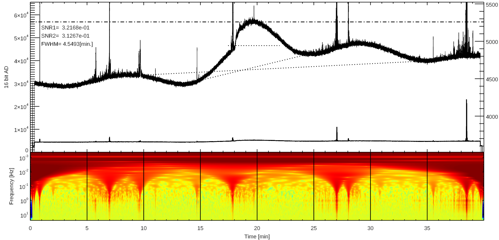
C 3C157 (/home4/archive/swift/dat/2025/10/T20251009043921.dat)
