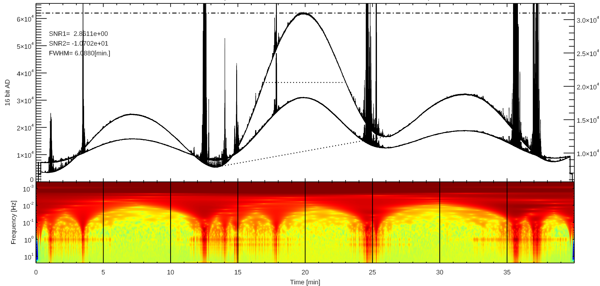
C 3C405 (/home4/archive/swift/dat/2025/10/T20251007182544.dat)
