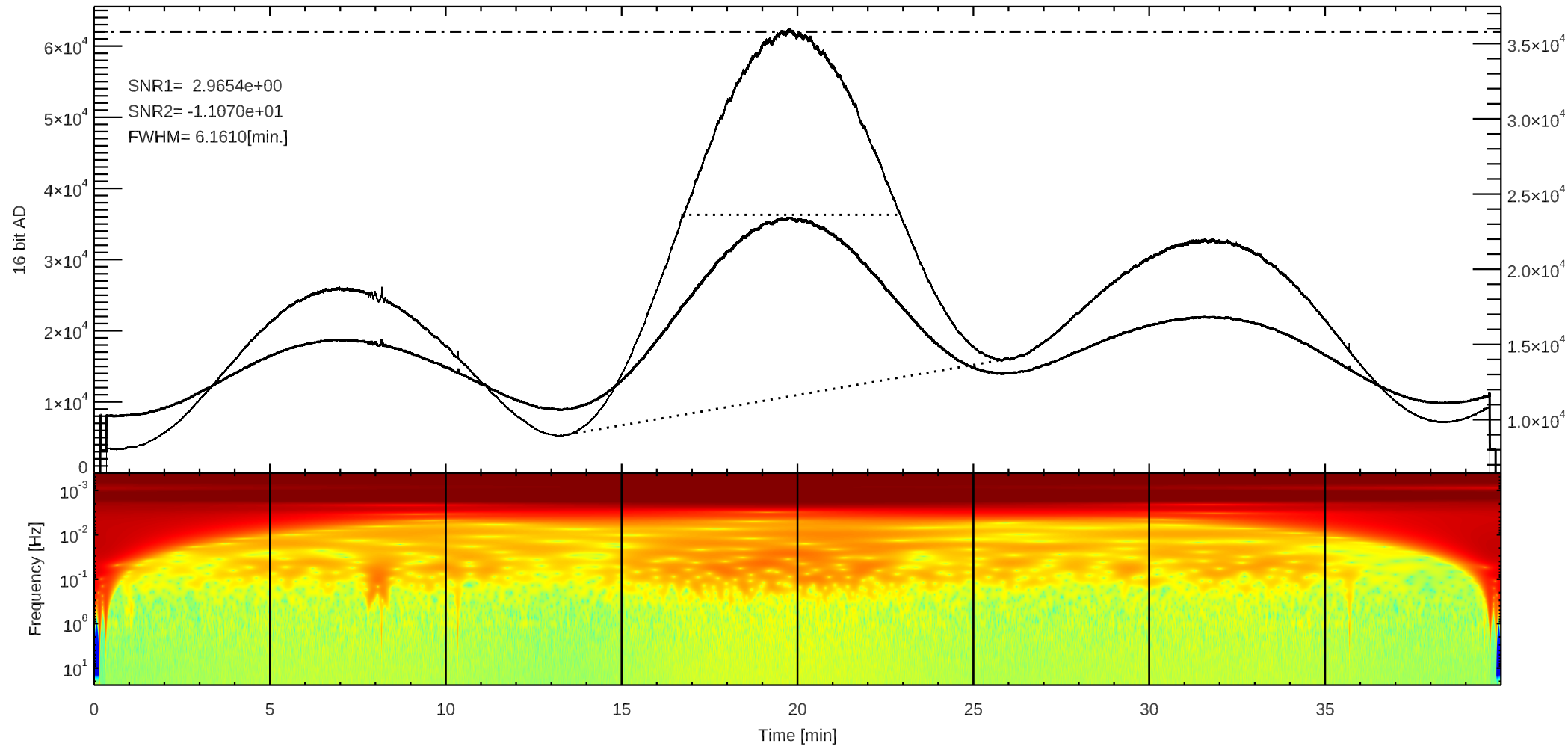
C 3C405 (/home4/archive/swift/dat/2025/10/T20251021173042.dat)
