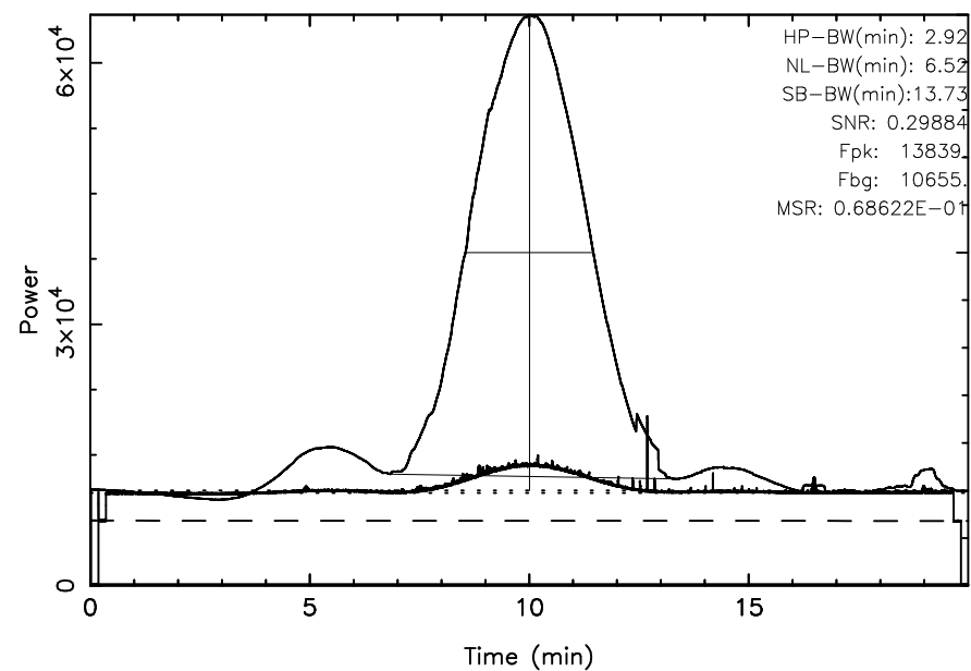
KISO 3C144 2025/10/11(284)03:58:01–04:18:01JST
