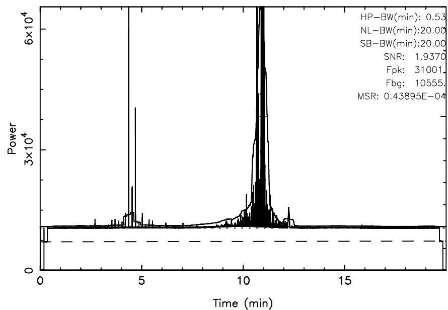
KISO 3C123 2025/10/11(284)03:00:49–03:20:49JST
