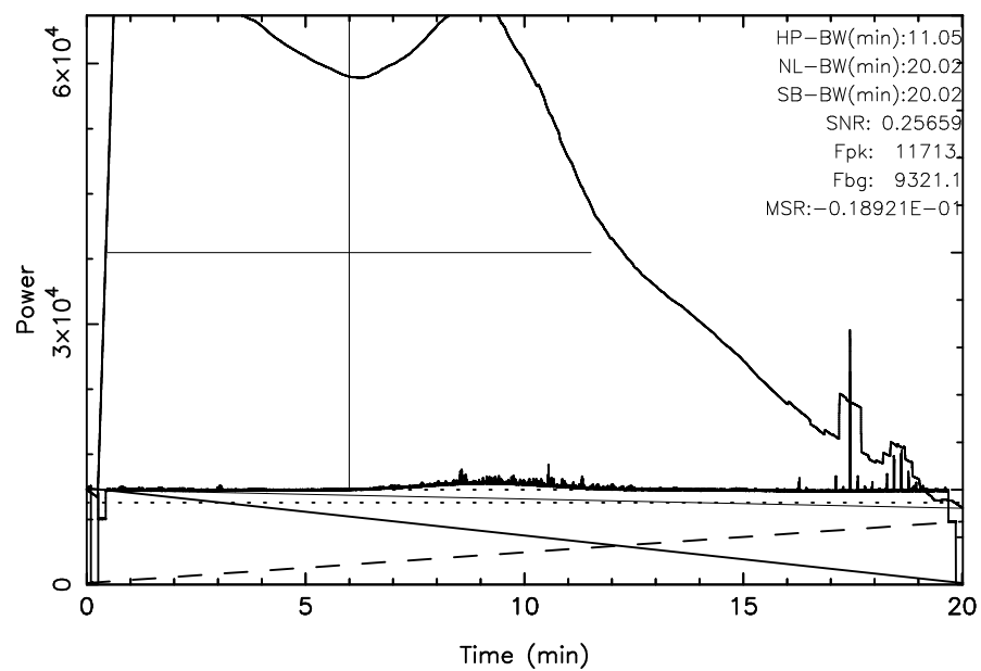
KISO 3C157 2025/10/11(284)04:41:26–05:01:27JST
