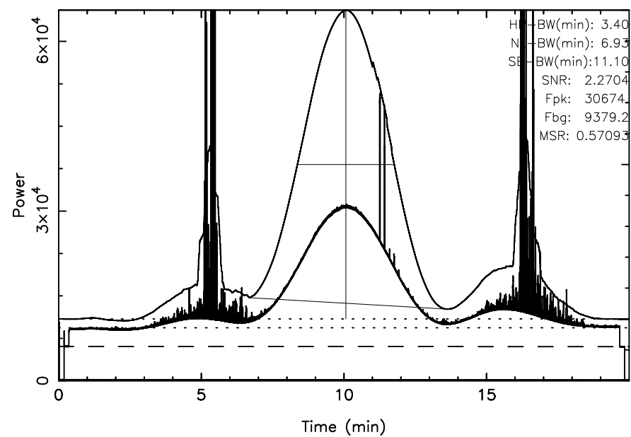
KISO 3C405 2025/10/11(284)18:19:59–18:39:59JST
