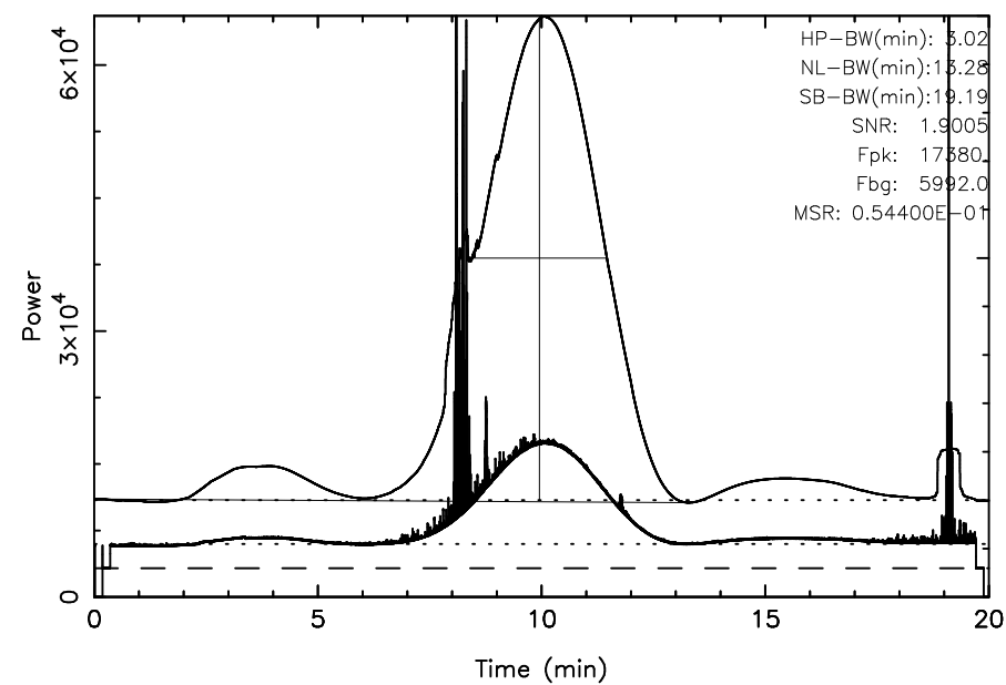
FUJI 3C405 2025/10/15(288)18:04:14-18:24:14JST
