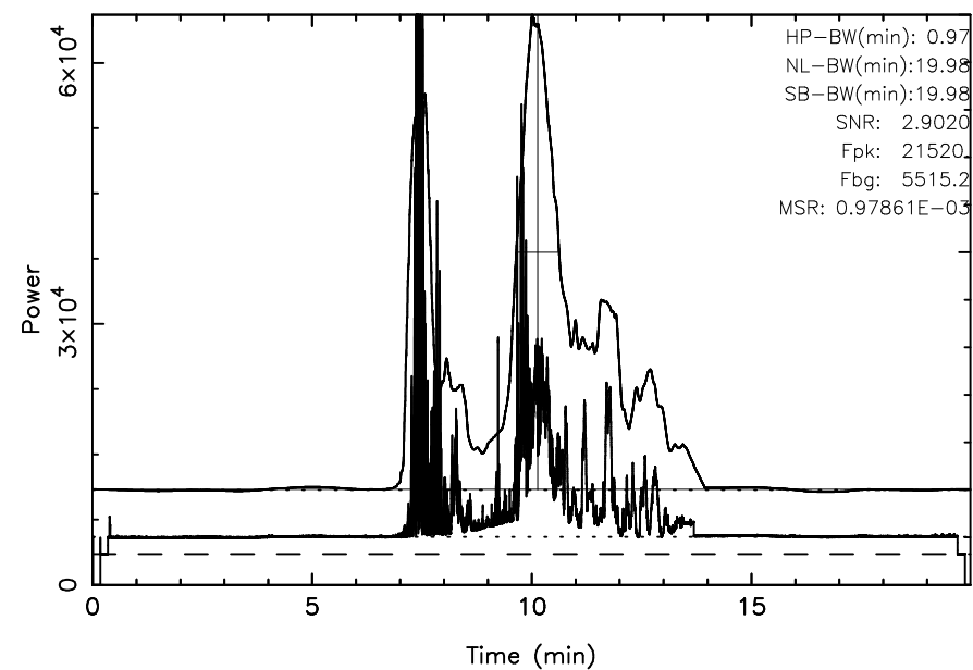
FUJI 3C144 2025/10/15(288)03:42:19-04:02:18JST
