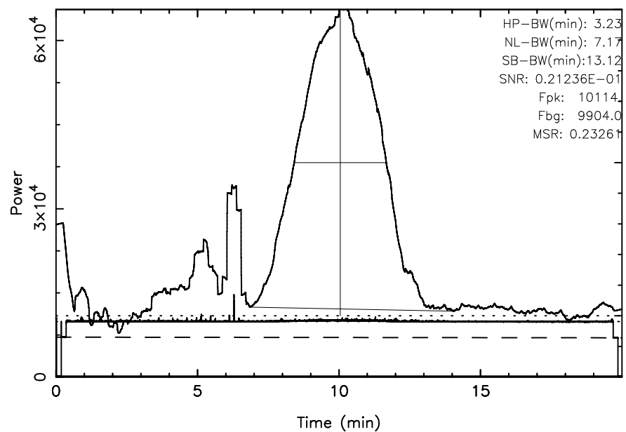
KISO 3C123 2025/10/15(288)02:45:05–03:05:05JST
