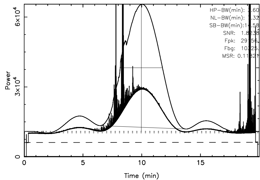
KISO 3C405 2025/10/15(288)18:04:14–18:24:14JST
