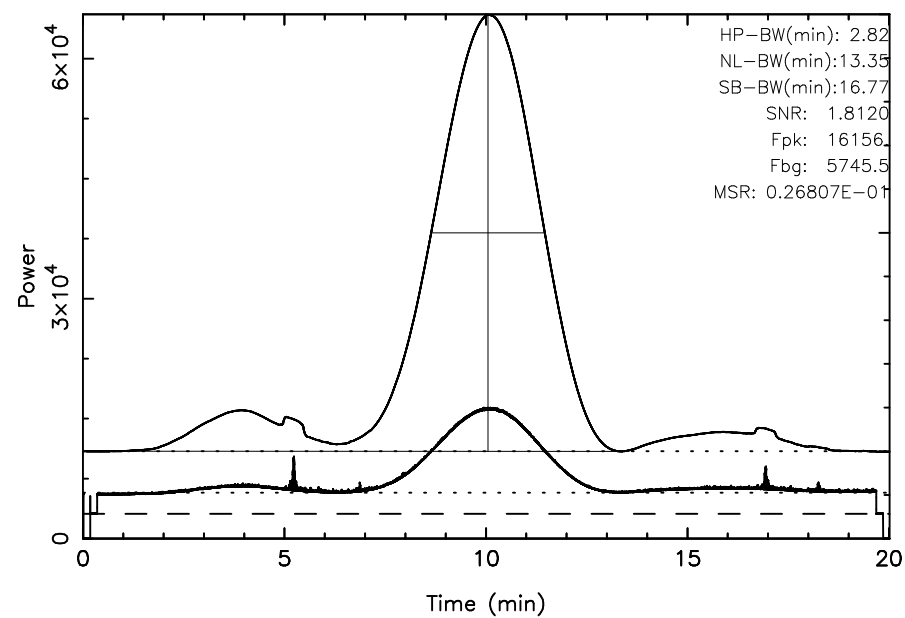
FUJI 3C405 2025/10/20(293)17:44:34-18:04:35JST
