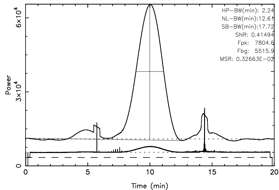
FUJI 3C144 2025/10/20(293)03:22:38-03:42:38JST
