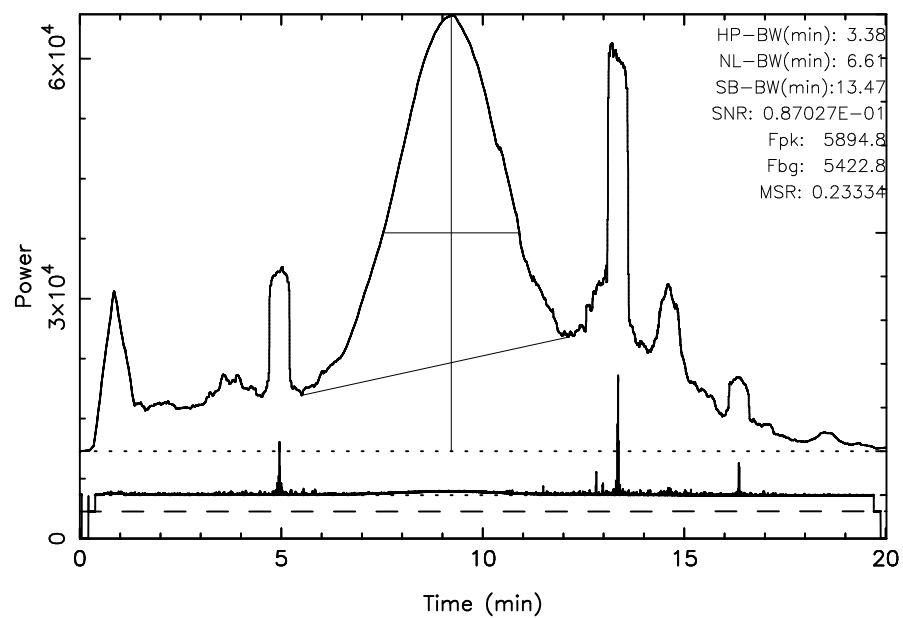
FUJI 3C157 2025/10/20(293)04:06:03-04:26:04JST
