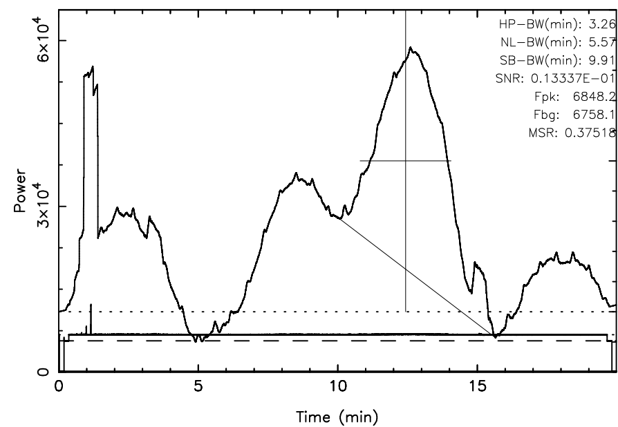
KISO 3C123 2025/10/24(297)02:09:43-02:29:42JST
