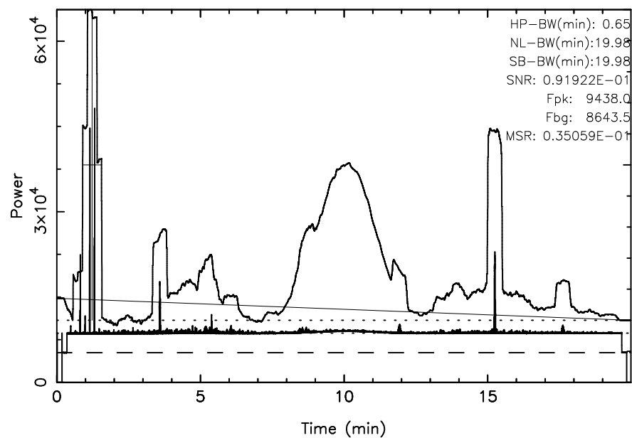
FUJI 3C123 2025/10/24(297)02:09:43-02:29:42JST
