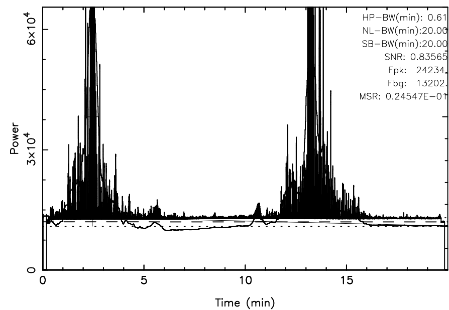
KISO 3C123 2025/10/29(302)01:50:04-02:10:04JST
