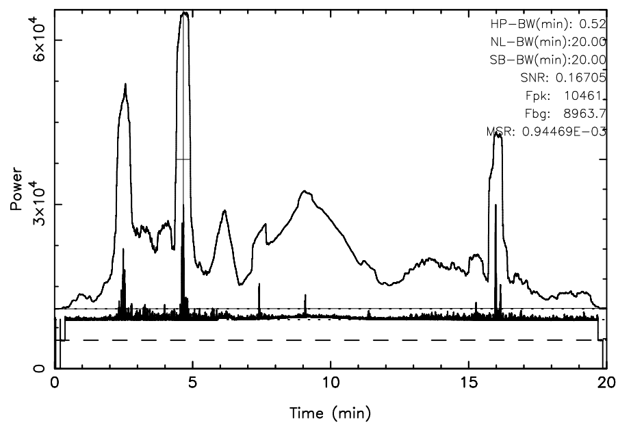
FUJI 3C157 2025/10/29(302)03:30:41-03:50:41JST
