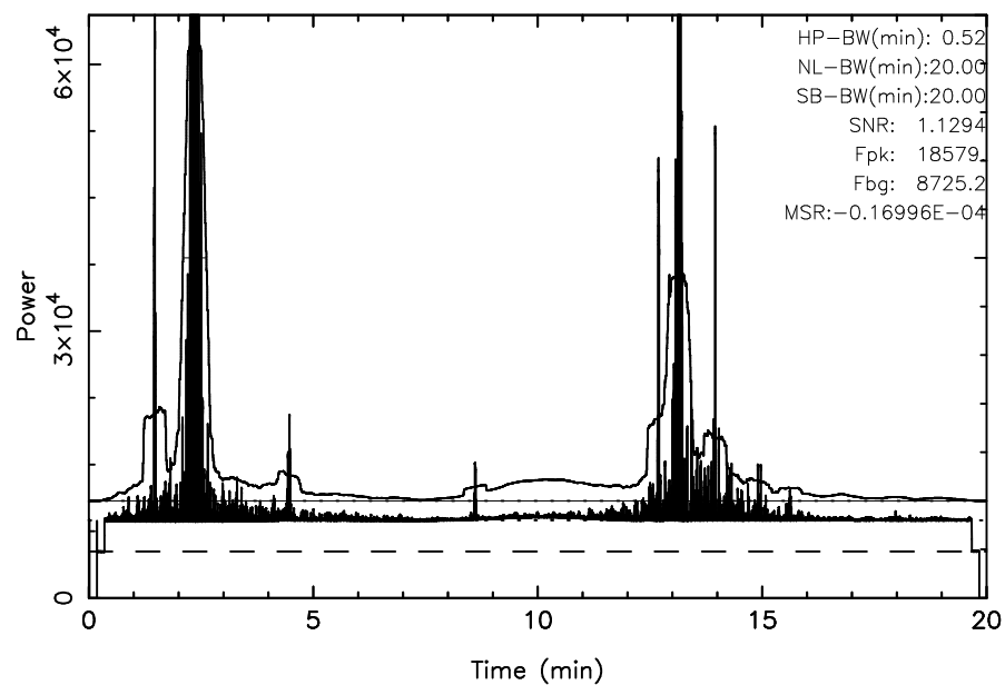
FUJI 3C123 2025/10/29(302)01:50:04-02:10:04JST
