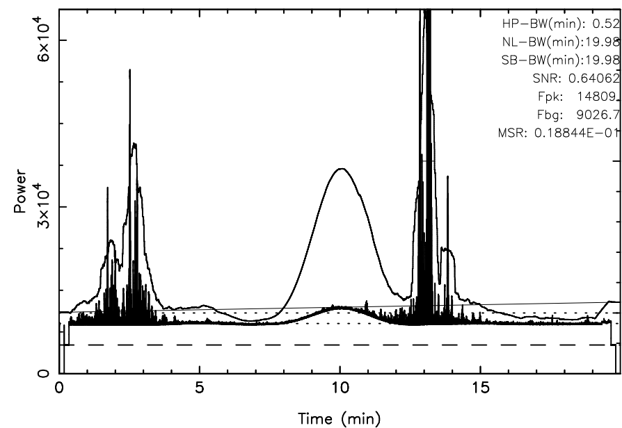
FUJI 3C144 2025/10/29(302)02:47:16-03:07:15JST
