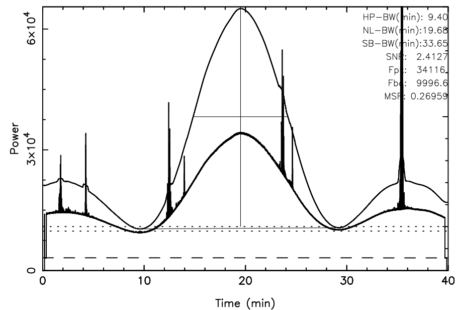
TOYOKAWA 3C461 2025/10/04(277)22:01:07–22:41:07JST
