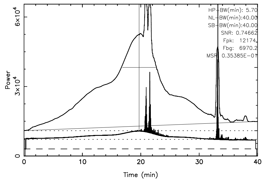
TOYOKAWA 3C392 2025/10/04(277)17:34:43-18:14:43JST
