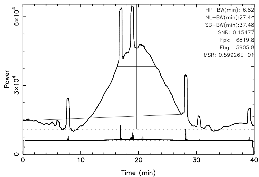
TOYOKAWA 3C10 2025/10/04(277)23:03:16–23:43:16JST
