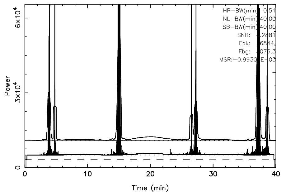
TOYOKAWA 3C123 2025/10/04(277)03:18:21-03:58:21JST
