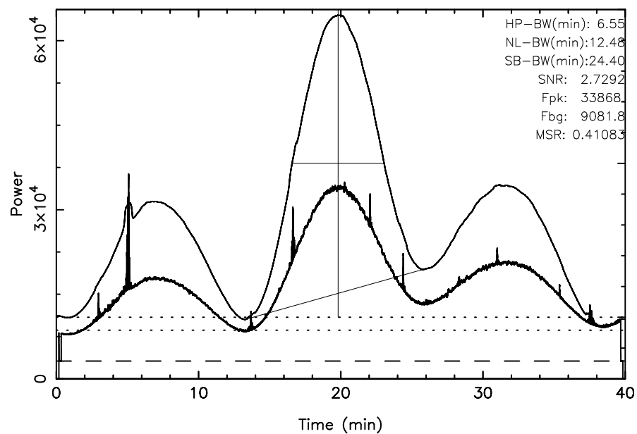
TOYOKAWA 3C405 2025/10/04(277)18:37:30–19:17:30JST
