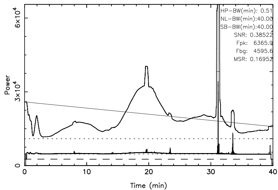
TOYOKAWA 3C157 2025/10/04(277)04:58:58-05:38:58JST
