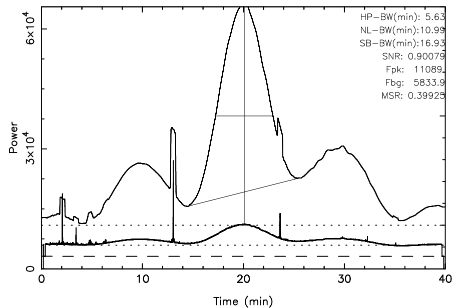
TOYOKAWA 3C144 2025/10/04(277)04:15:34-04:55:34JST
