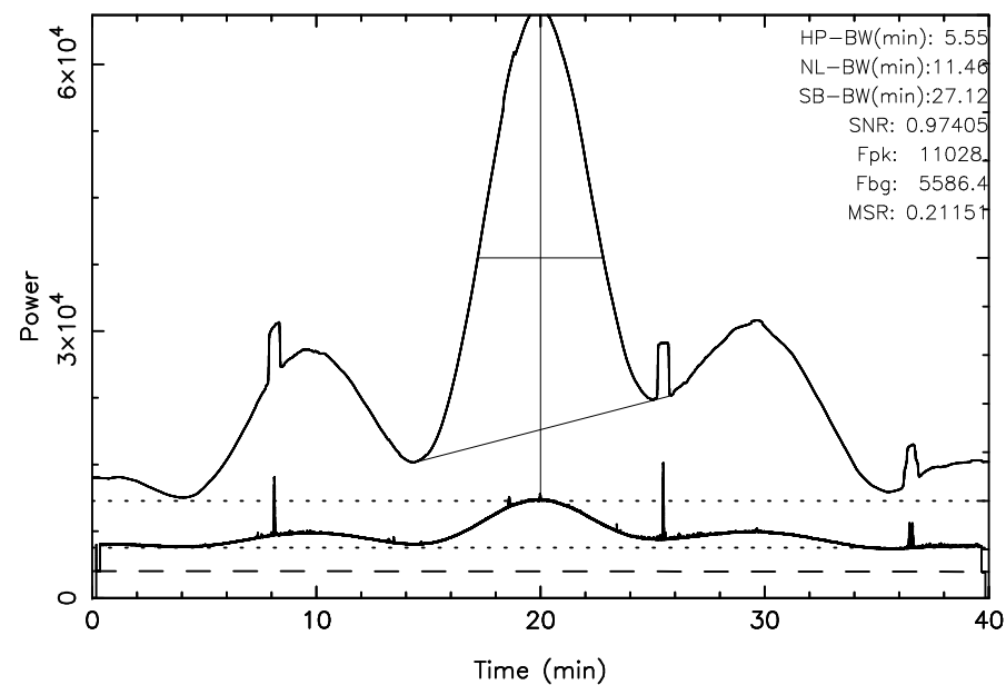
TOYOKAWA 3C144 2025/10/05(278)04:11:38-04:51:38JST
