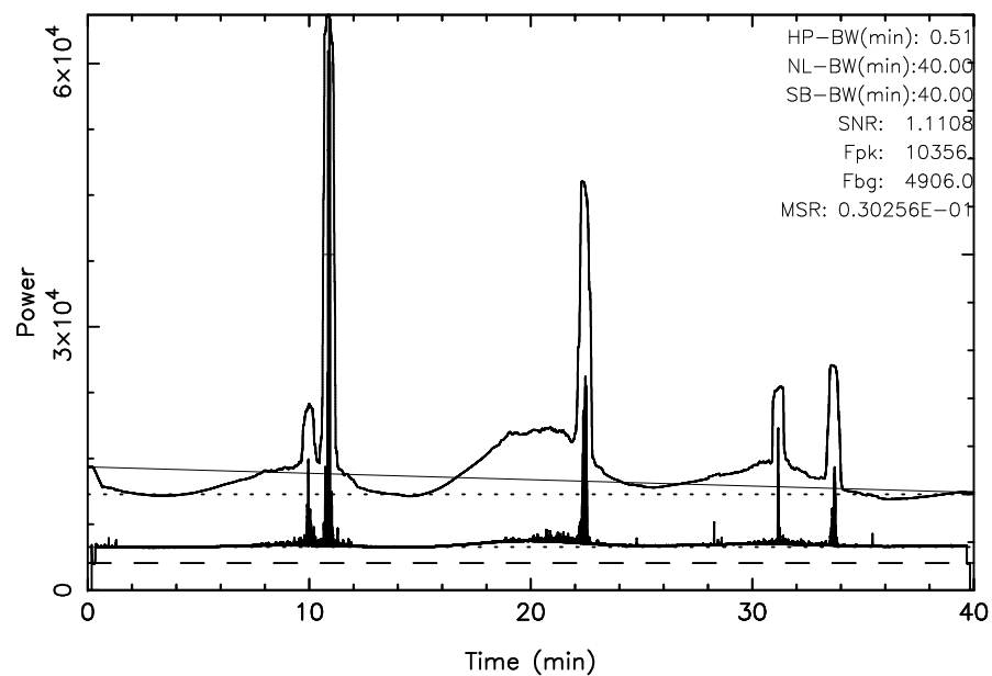
TOYOKAWA 3C123 2025/10/05(278)03:14:25-03:54:25JST
