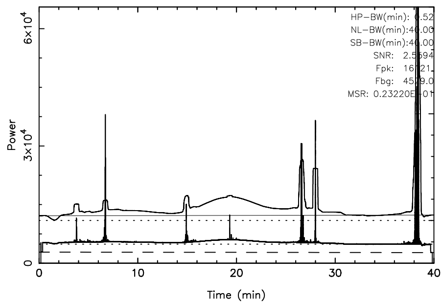
TOYOKAWA 3C157 2025/10/05(278)04:55:02-05:35:02JST
