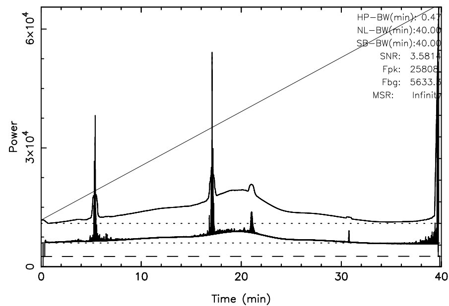
TOYOKAWA 3C392 2025/10/05(278)17:30:47-18:10:47JST
