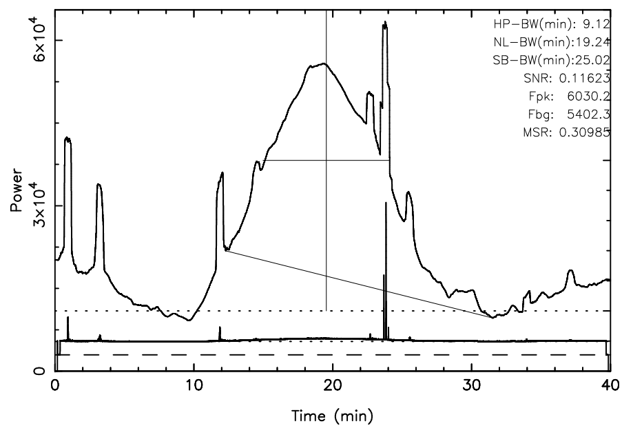
TOYOKAWA 3C10 2025/10/05(278)22:59:20–23:39:20JST
