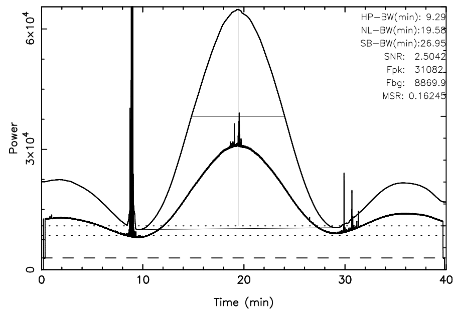
TOYOKAWA 3C461 2025/10/05(278)21:57:11–22:37:11JST
