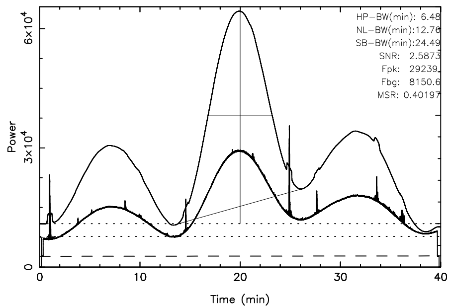
TOYOKAWA 3C405 2025/10/05(278)18:33:34–19:13:34JST
