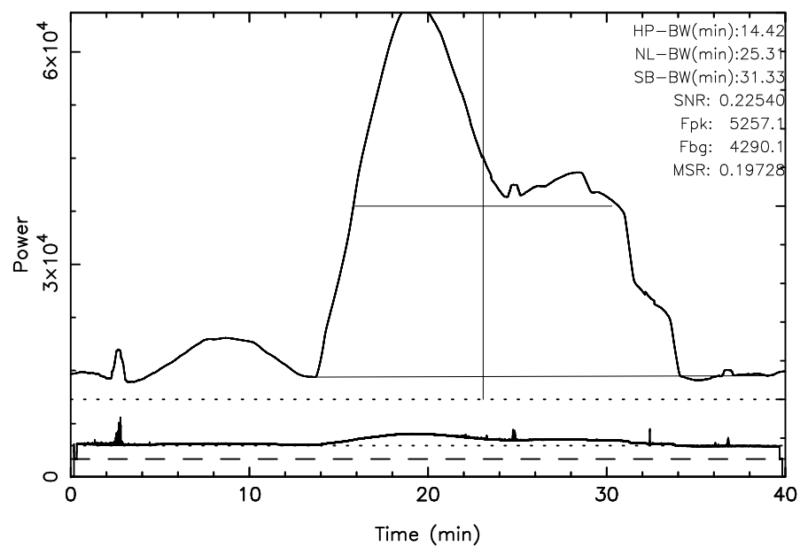
TOYOKAWA 3C157 2025/10/16(289)04:11:47–04:51:47JST
