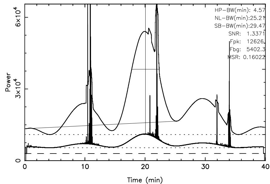
TOYOKAWA 3C144 2025/10/16(289)03:28:23–04:08:23JST
