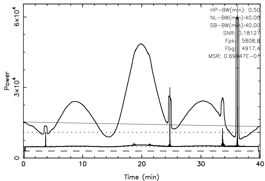
TOYOKAWA 3C123 2025/10/16(289)02:31:10–03:11:10JST
