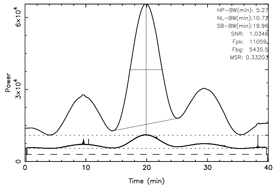
TOYOKAWA 3C144 2025/10/19(292)03:16:35-03:56:35JST
