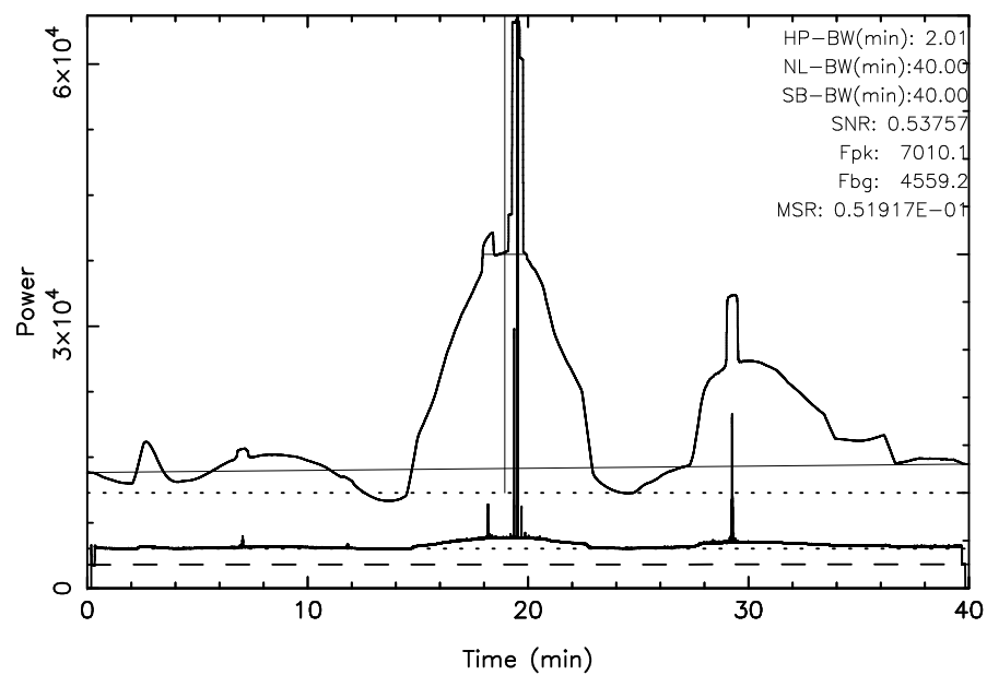
TOYOKAWA 3C157 2025/10/19(292)04:00:00-04:40:00JST
