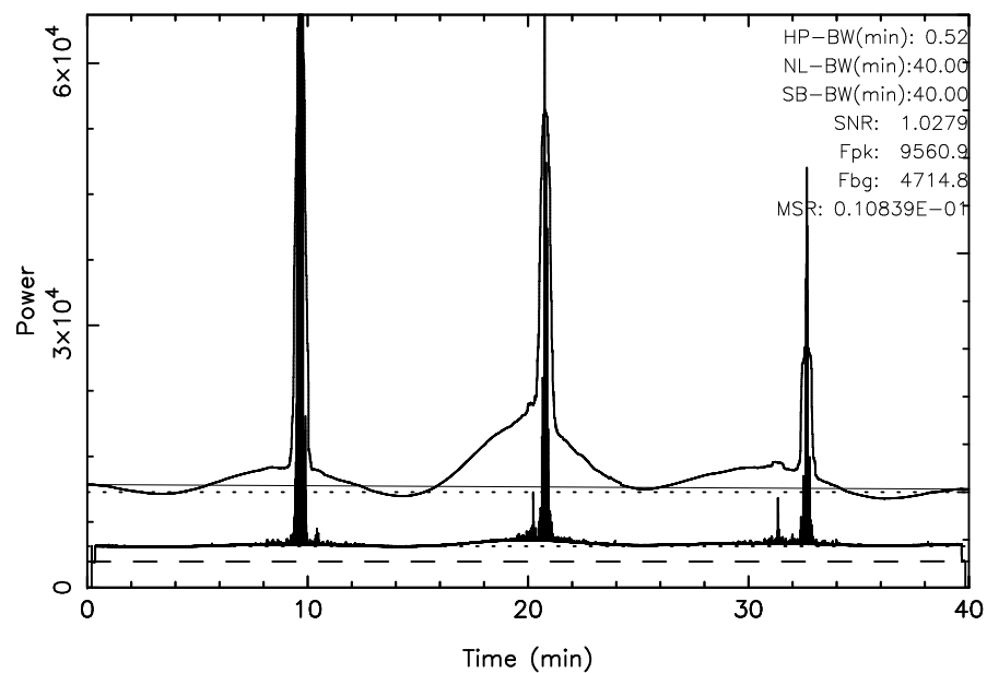
TOYOKAWA 3C123 2025/10/19(292)02:19:23-02:59:23JST
