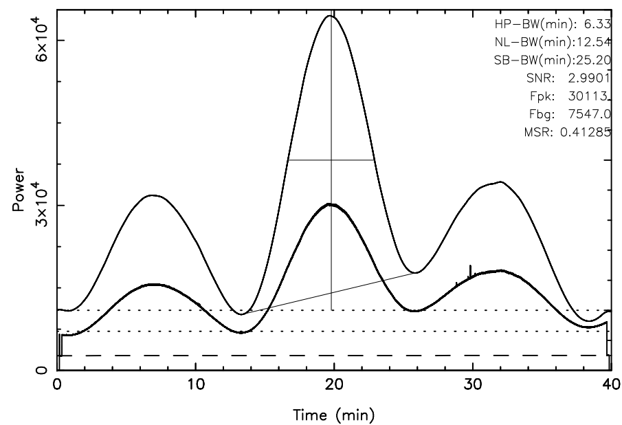
TOYOKAWA 3C405 2025/10/19(292)17:38:31-18:18:31JST
