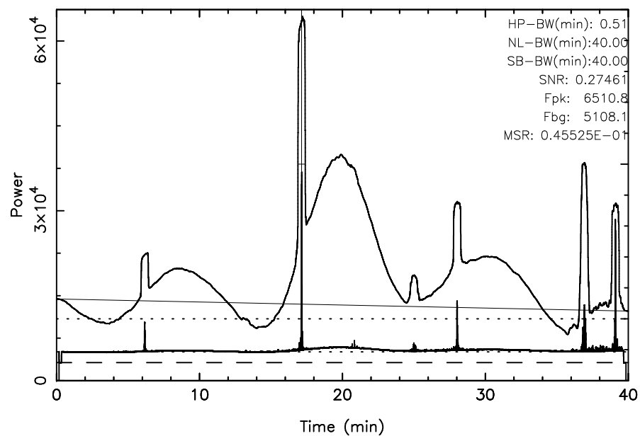
TOYOKAWA 3C123 2025/10/26(299)01:51:51-02:31:51JST
