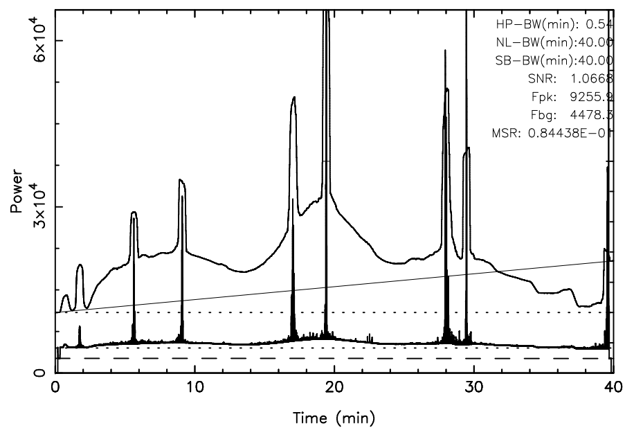
TOYOKAWA 3C157 2025/10/26(299)03:32:28-04:12:28JST
