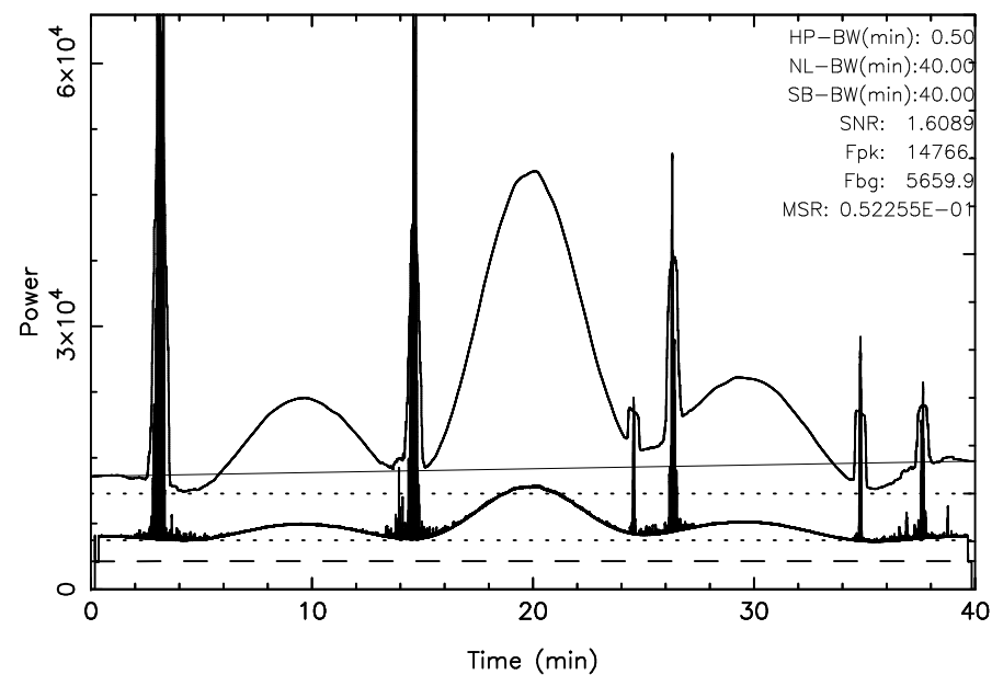
TOYOKAWA 3C144 2025/10/26(299)02:49:04-03:29:04JST
