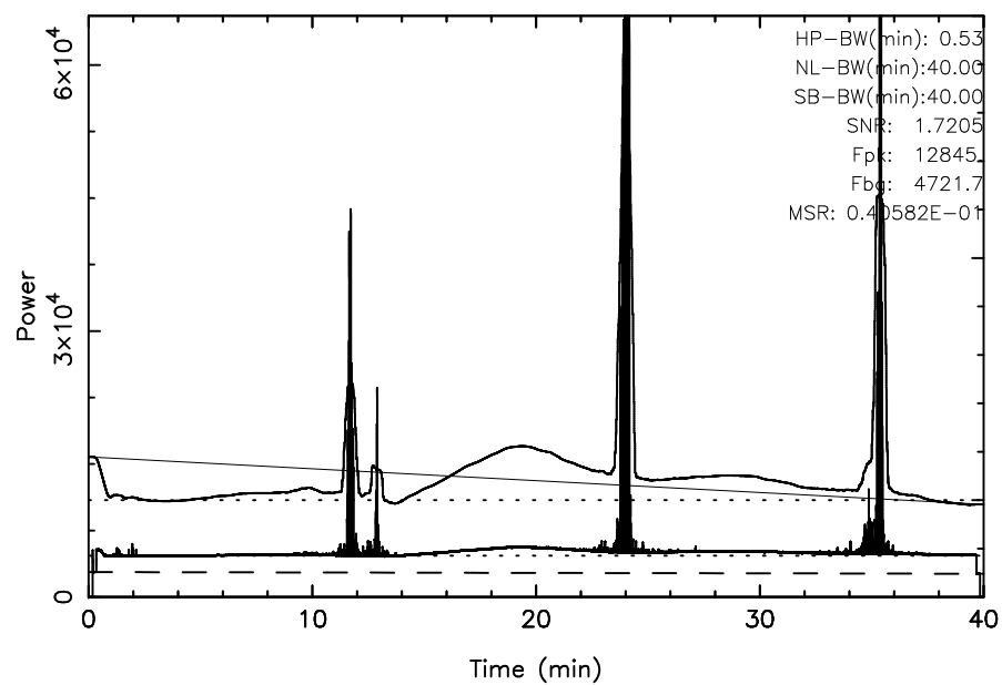
TOYOKAWA 3C157 2025/10/27(300)03:28:32-04:08:32JST
