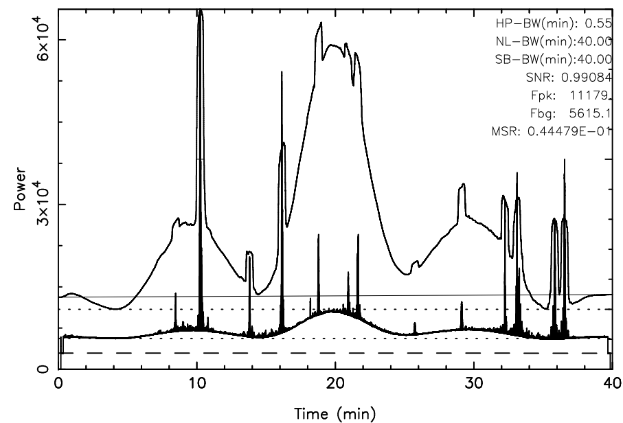
TOYOKAWA 3C144 2025/10/27(300)02:45:08-03:25:08JST
