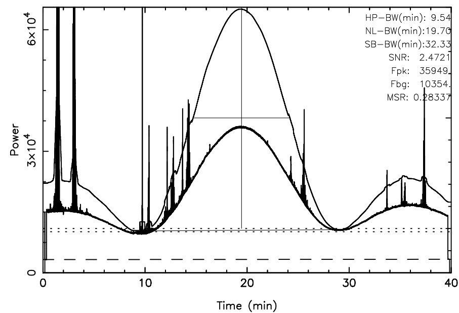
TOYOKAWA 3C461 2025/10/27(300)20:30:41-21:10:41JST
