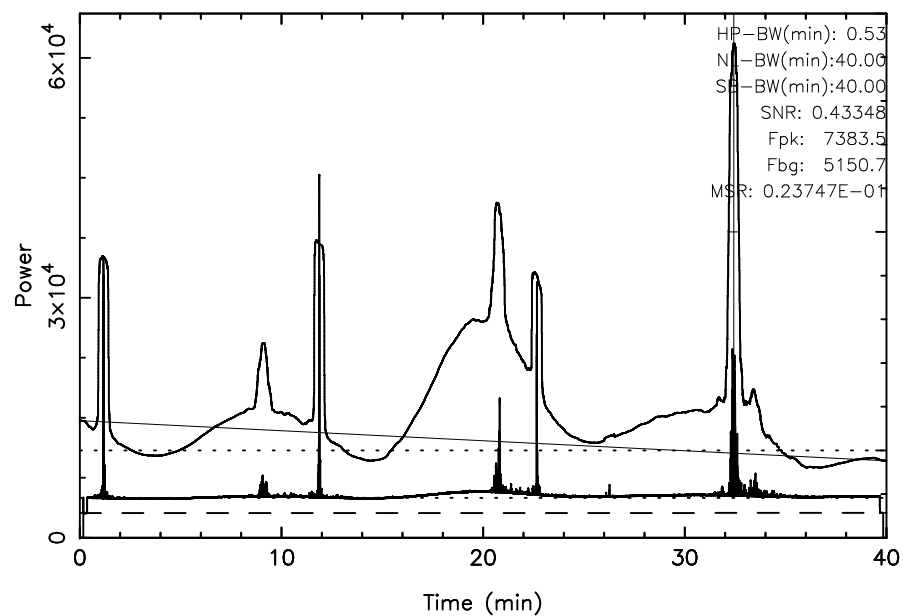
TOYOKAWA 3C123 2025/10/27(300)01:47:56-02:27:56JST
