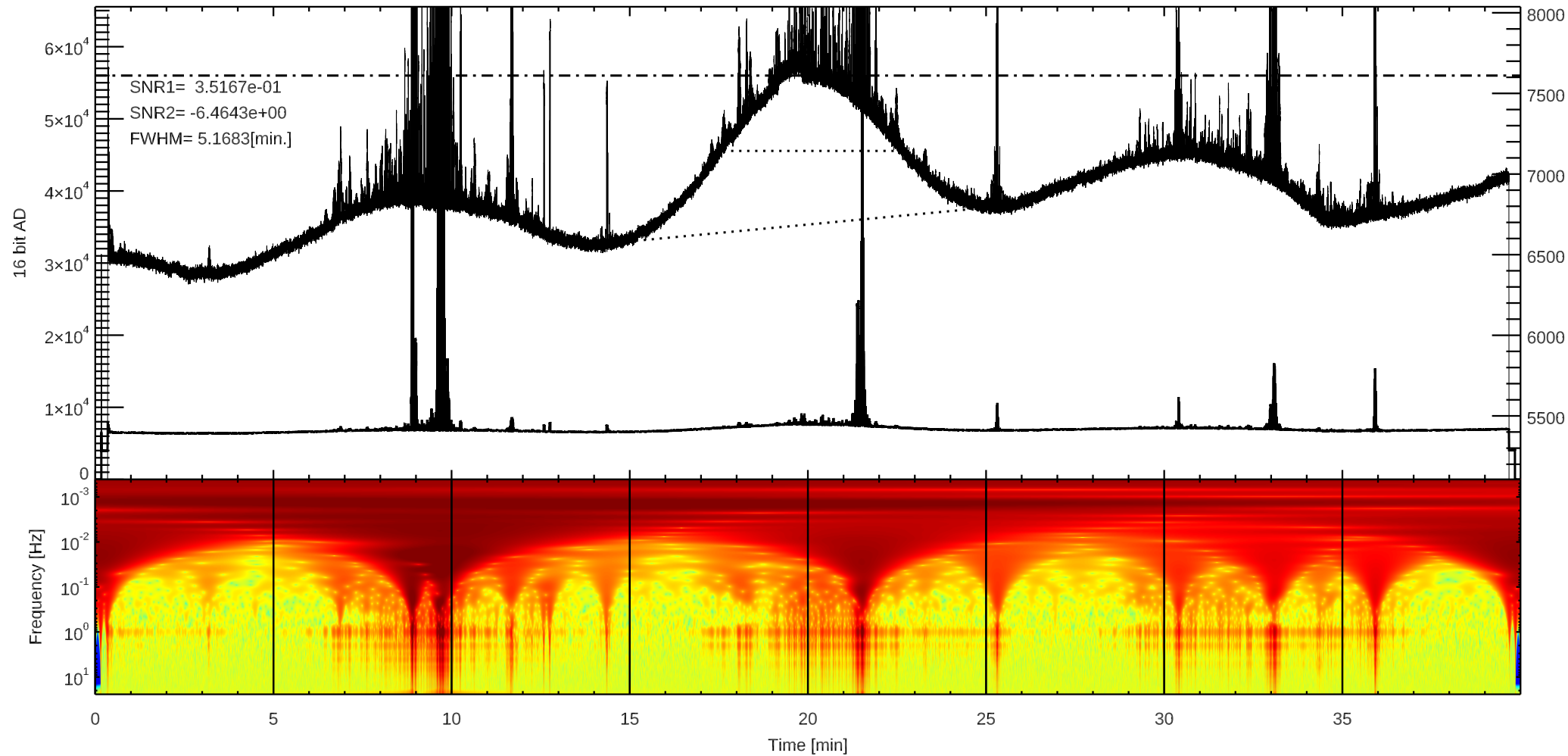
C 3C123 (/home4/archive/swift/dat/2025/11/T20251103012026.dat)
