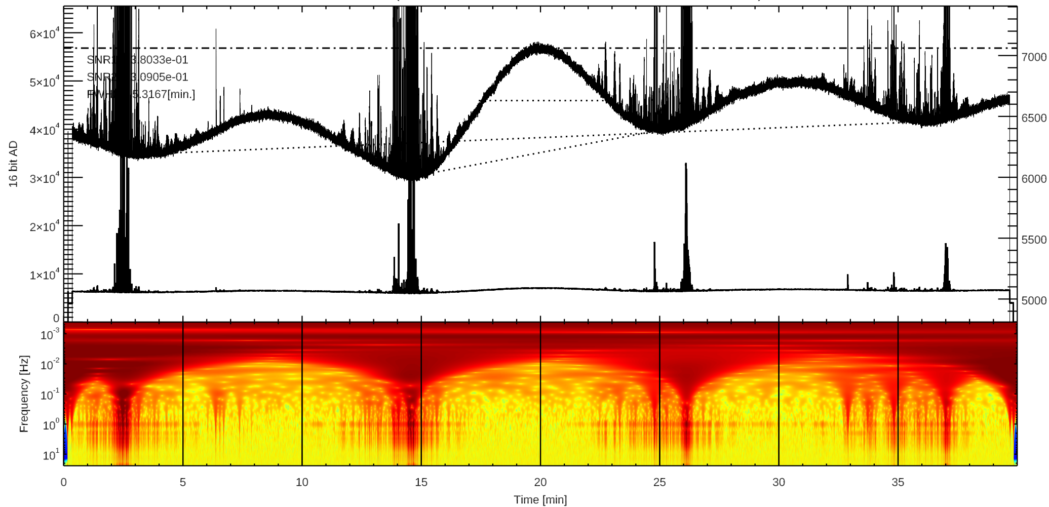
C 3C123 (/home4/archive/swift/dat/2025/11/T20251112004503.dat)
