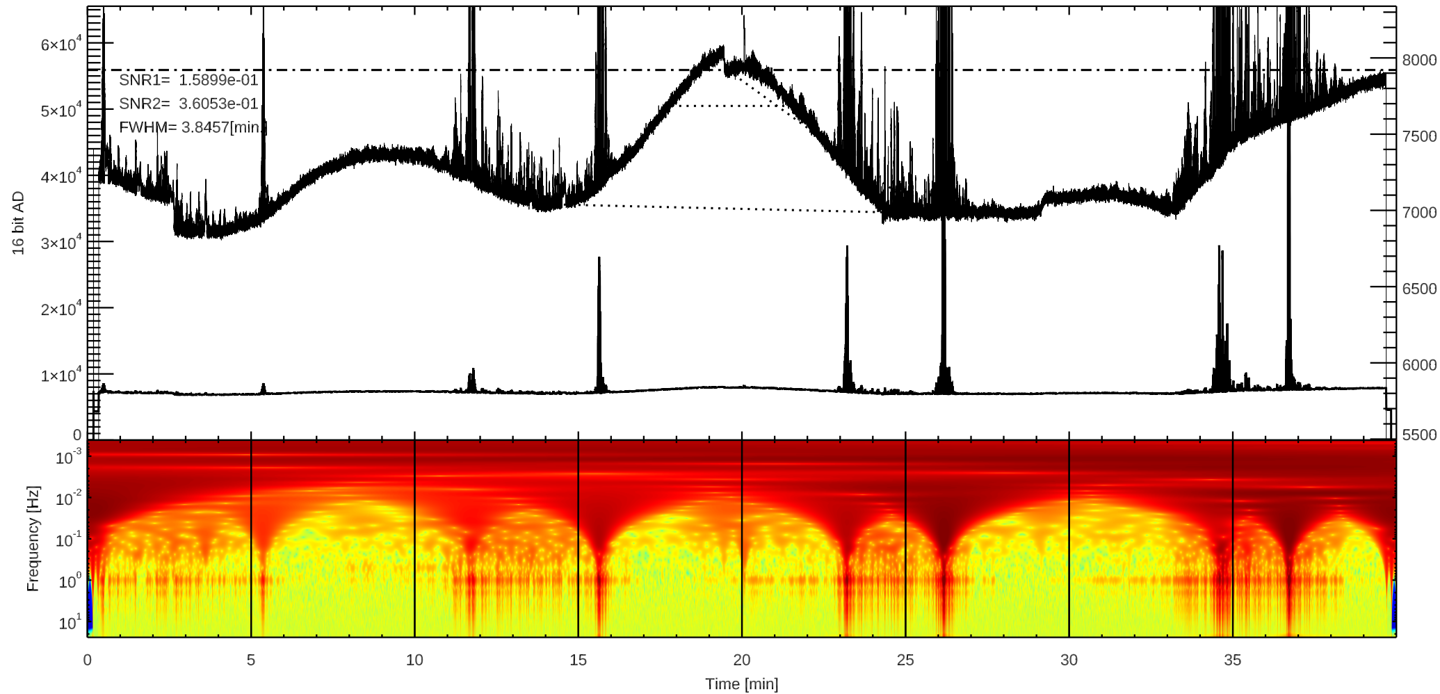
C 3C123 (/home4/archive/swift/dat/2025/11/T20251119001732.dat)
