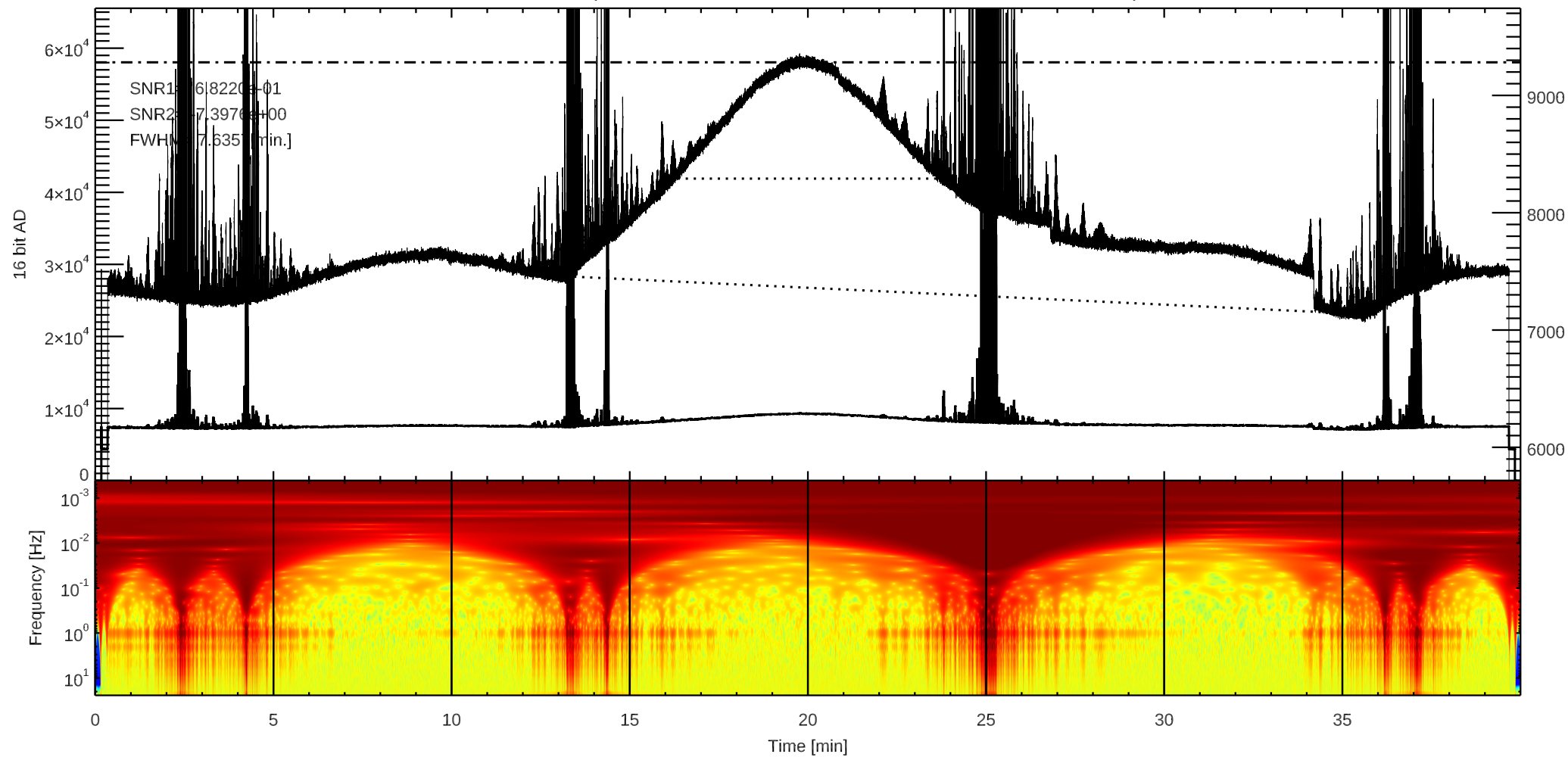
C 3C123 (/home4/archive/swift/dat/2025/11/T20251121000940.dat)
