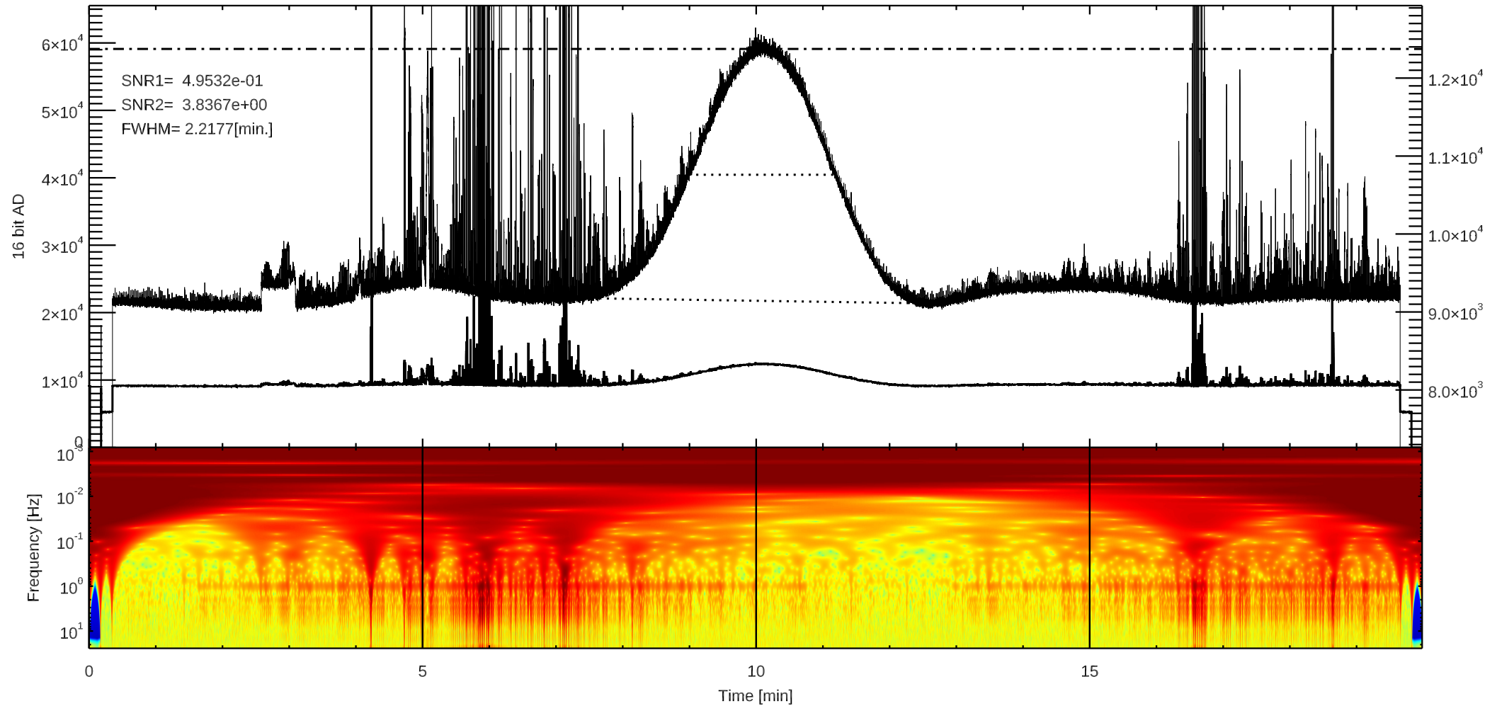
C 3C144 (/home4/archive/fit/dat/2025/11/F20251109020403.dat)
