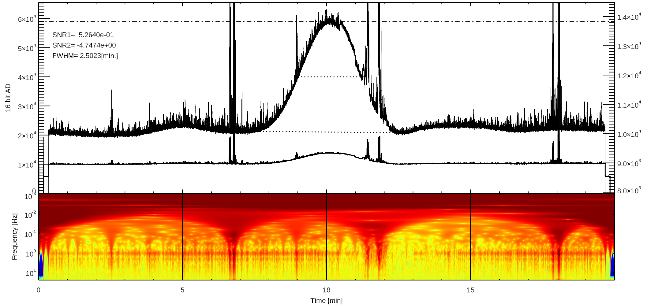
C 3C144 (/home4/archive/fit/dat/2025/11/F20251111015610.dat)
