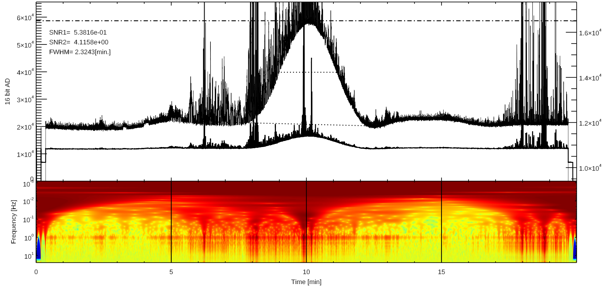
C 3C144 (/home4/archive/fit/dat/2025/11/F20251129004525.dat)
