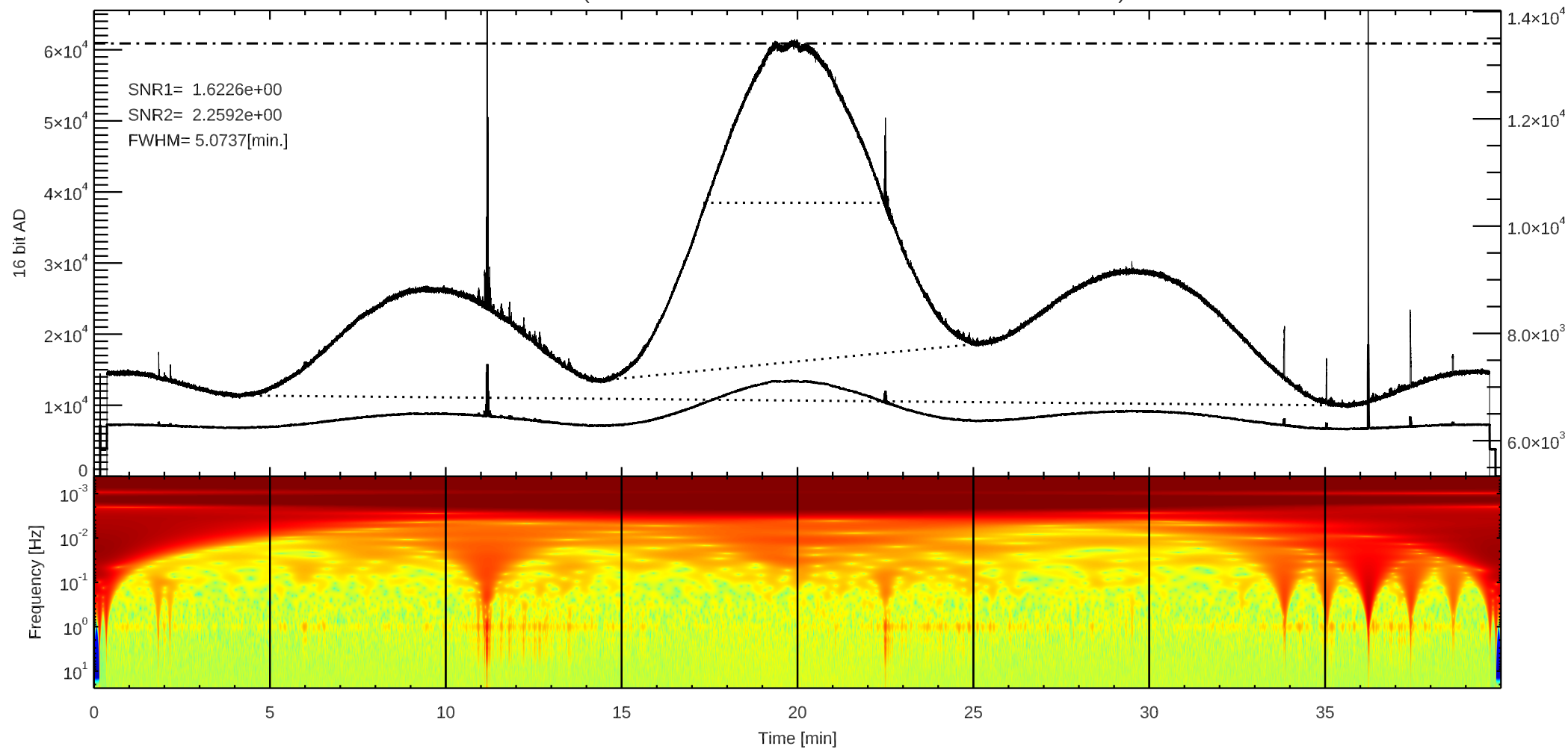
C 3C144 (/home4/archive/swift/dat/2025/11/T20251112014216.dat)
