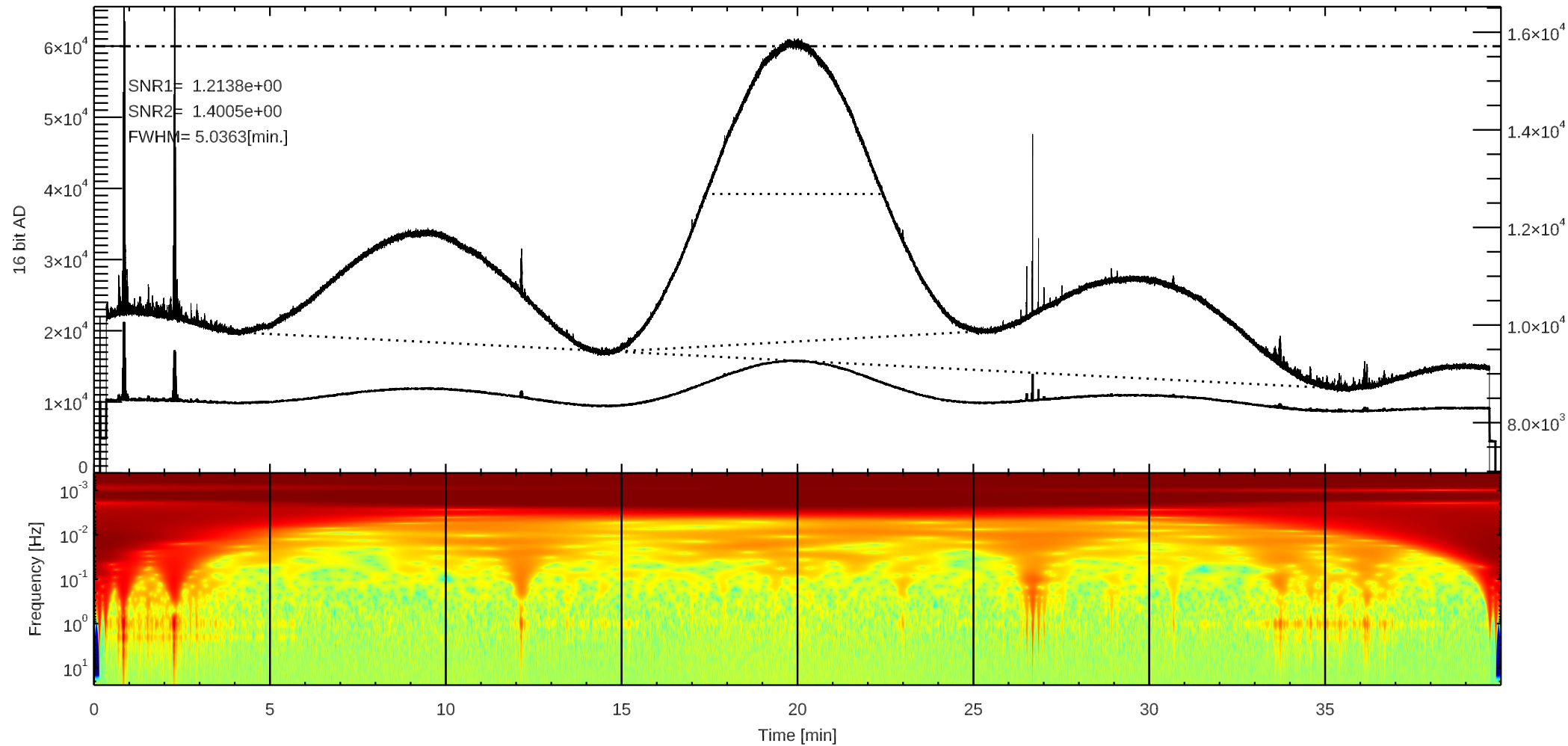
C 3C144 (/home4/archive/swift/dat/2025/11/T20251123005901.dat)
