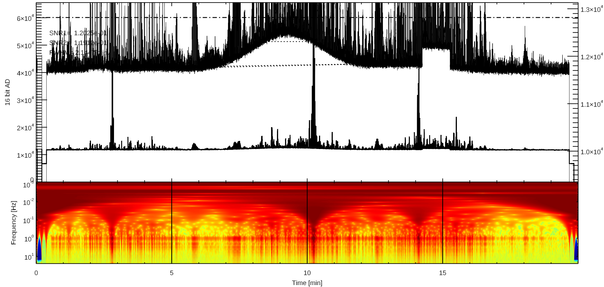
C 3C157 (/home4/archive/fit/dat/2025/11/F20251123015224.dat)
