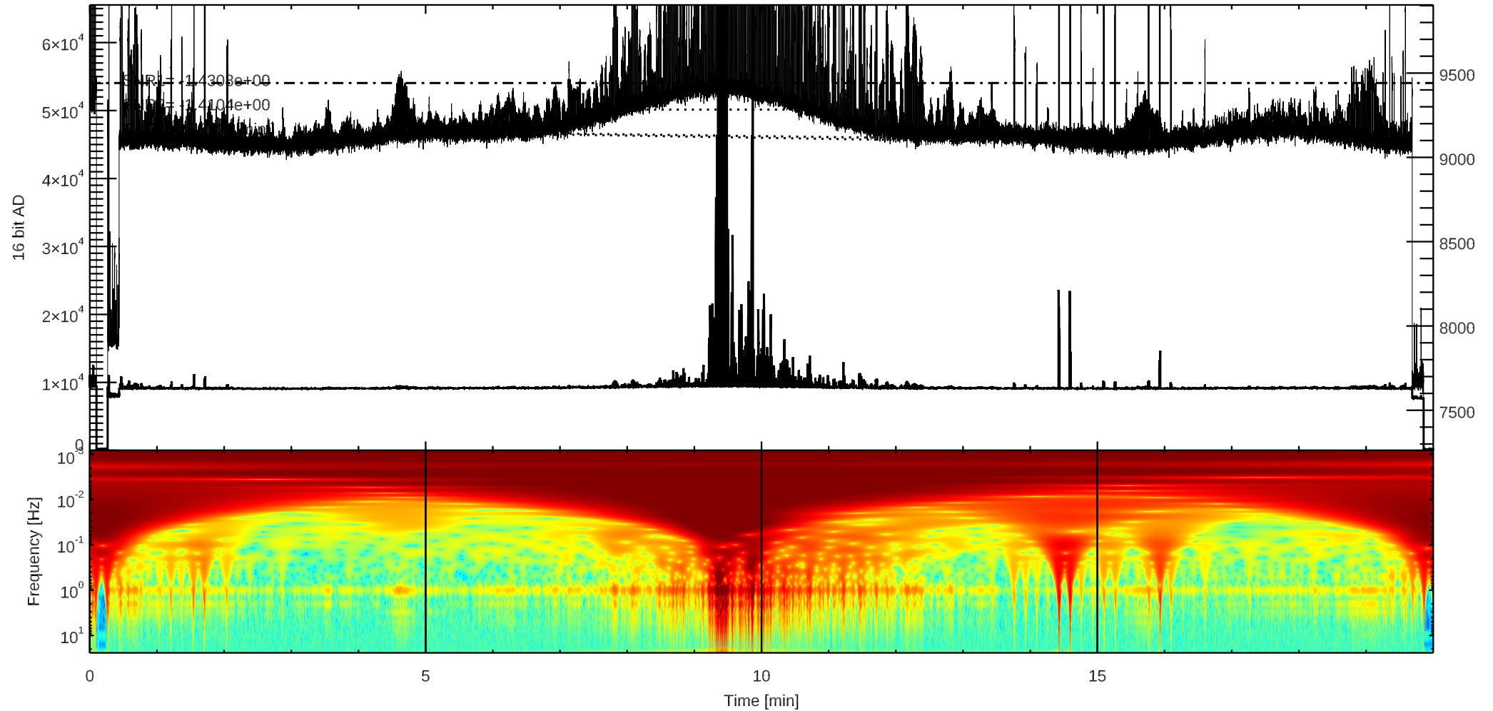
C 3C157 (/home4/archive/kit/dat/2025/11/K20251102031458.dat)
