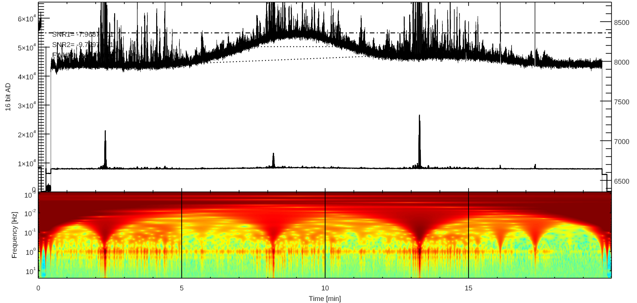
C 3C157 (/home4/archive/kit/dat/2025/11/K20251110024331.dat)
