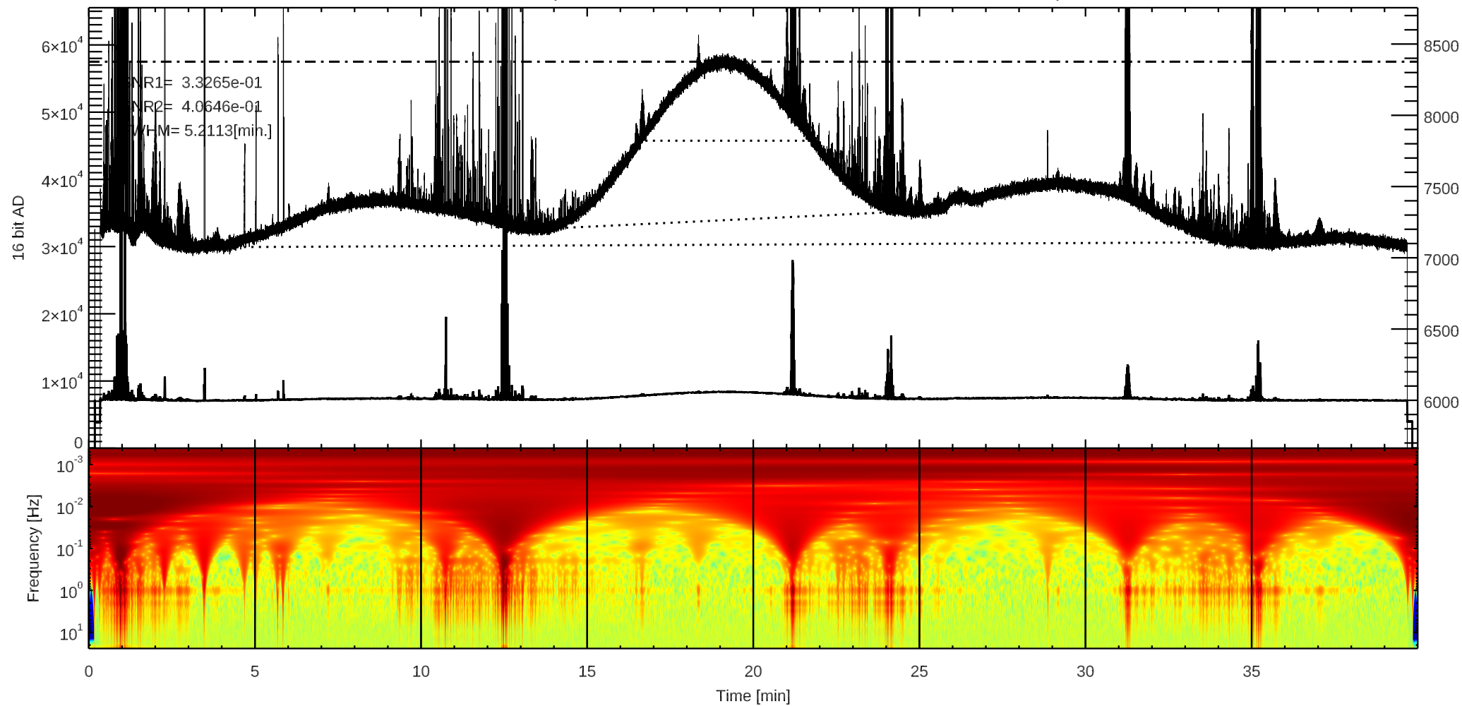
C 3C157 (/home4/archive/swift/dat/2025/11/T20251103030103.dat)
