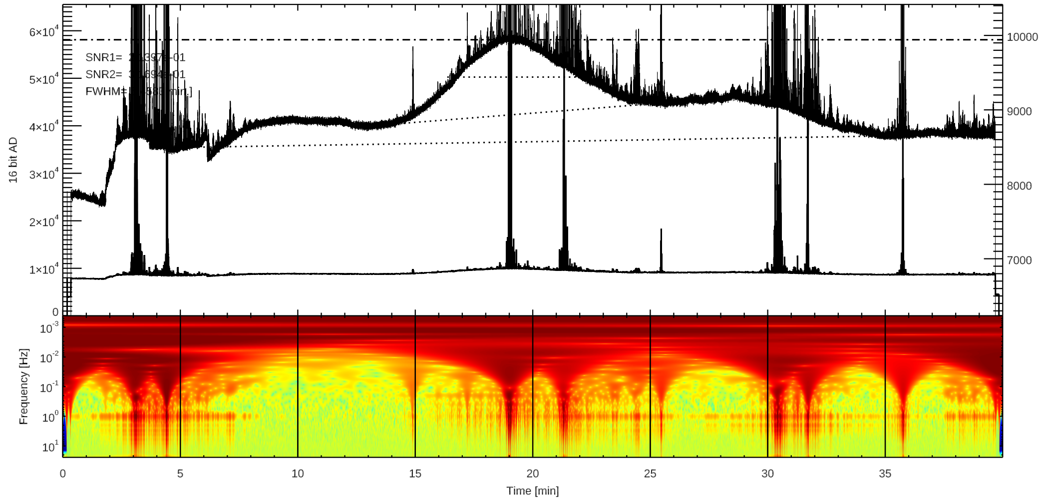
C 3C157 (/home4/archive/swift/dat/2025/11/T20251124013829.dat)
