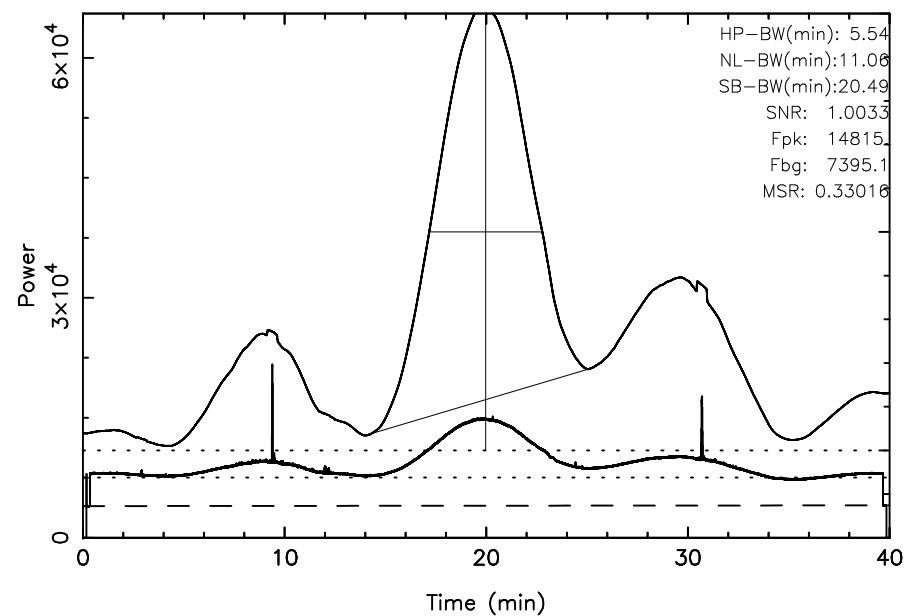
TOYOKAWA 3C144 2025/11/11(315)01:46:09-02:26:09JST
