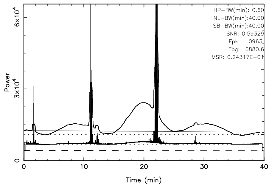
TOYOKAWA 3C123 2025/11/11(315)00:48:57-01:28:57JST
