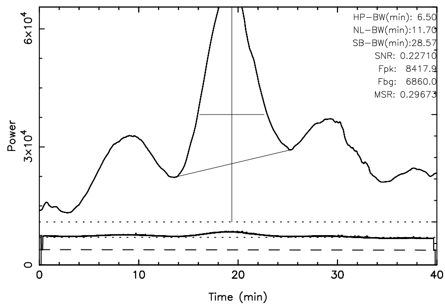
TOYOKAWA 3C157 2025/11/11(315)02:29:34-03:09:34JST
