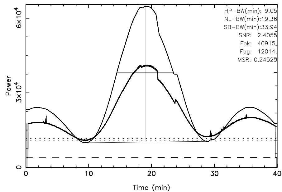
TOYOKAWA 3C461 2025/11/11(315)19:31:43-20:11:43JST
