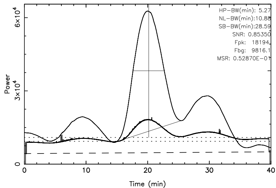
TOYOKAWA 3C144 2025/11/24(328)00:55:03–01:35:03JST
