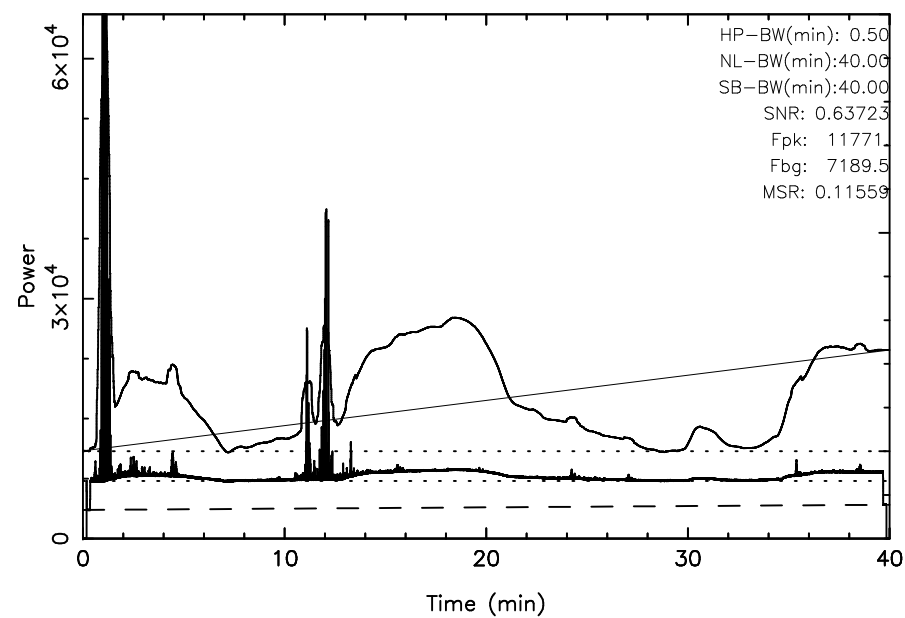
TOYOKAWA 3C10 2025/11/24(328)19:42:45–20:22:45JST
