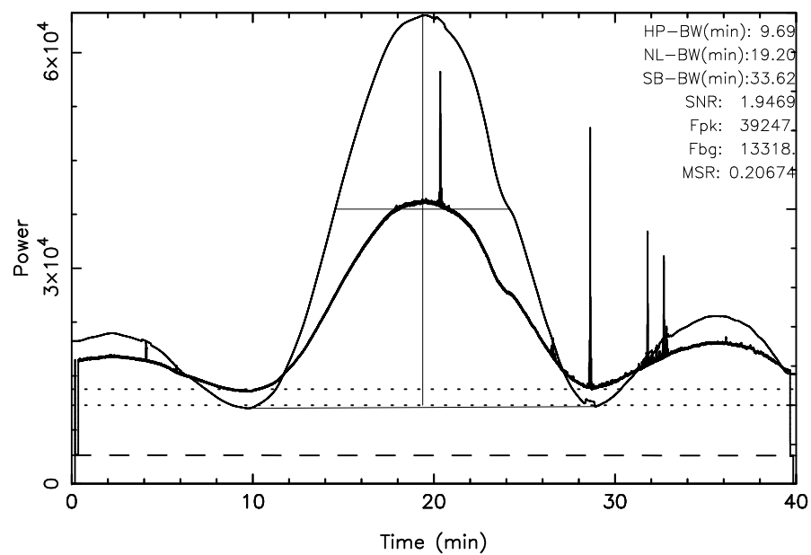
TOYOKAWA 3C461 2025/11/24(328)18:40:36–19:20:36JST
