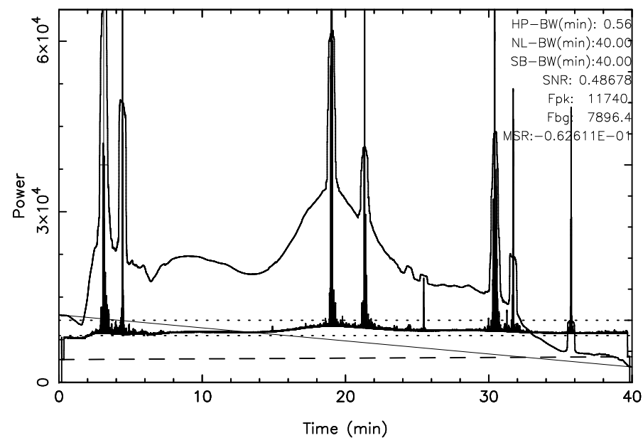
TOYOKAWA 3C157 2025/11/24(328)01:38:27–02:18:27JST
