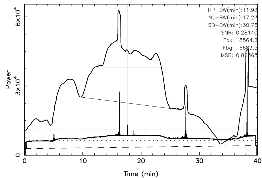
TOYOKAWA 3C10 2025/11/29(333)19:23:06-20:03:06JST
