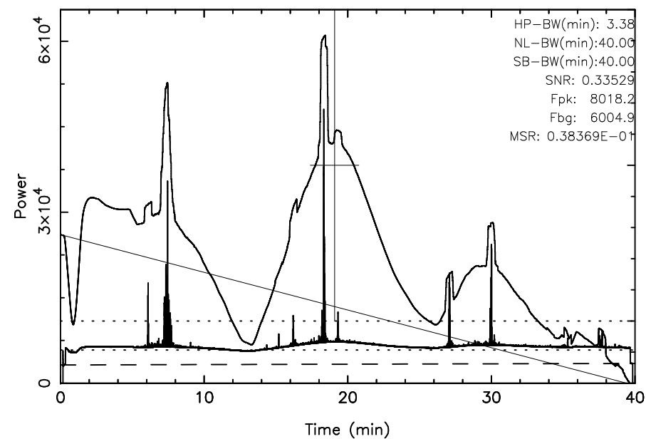
TOYOKAWA 3C157 2025/11/29(333)01:18:48-01:58:48JST
