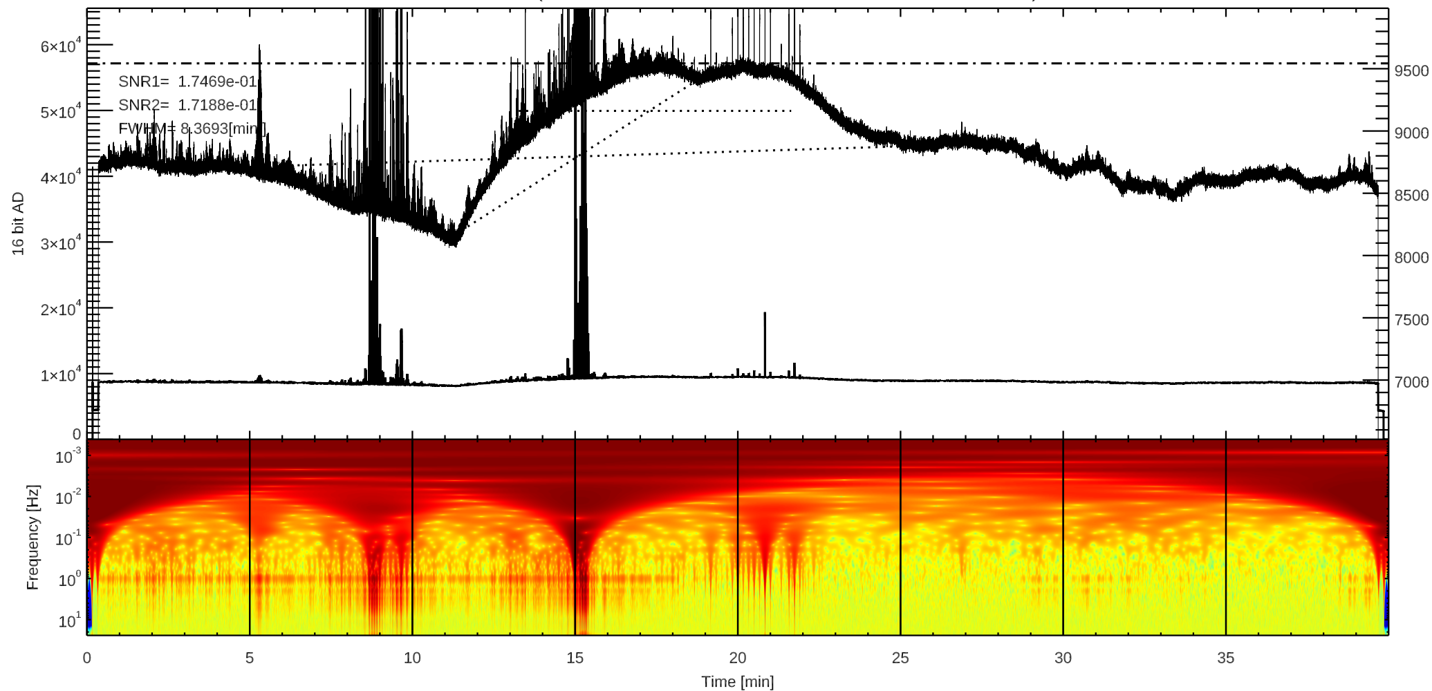
C 3C10 (/home4/archive/swift/dat/2025/12/T20251217181222.dat)
