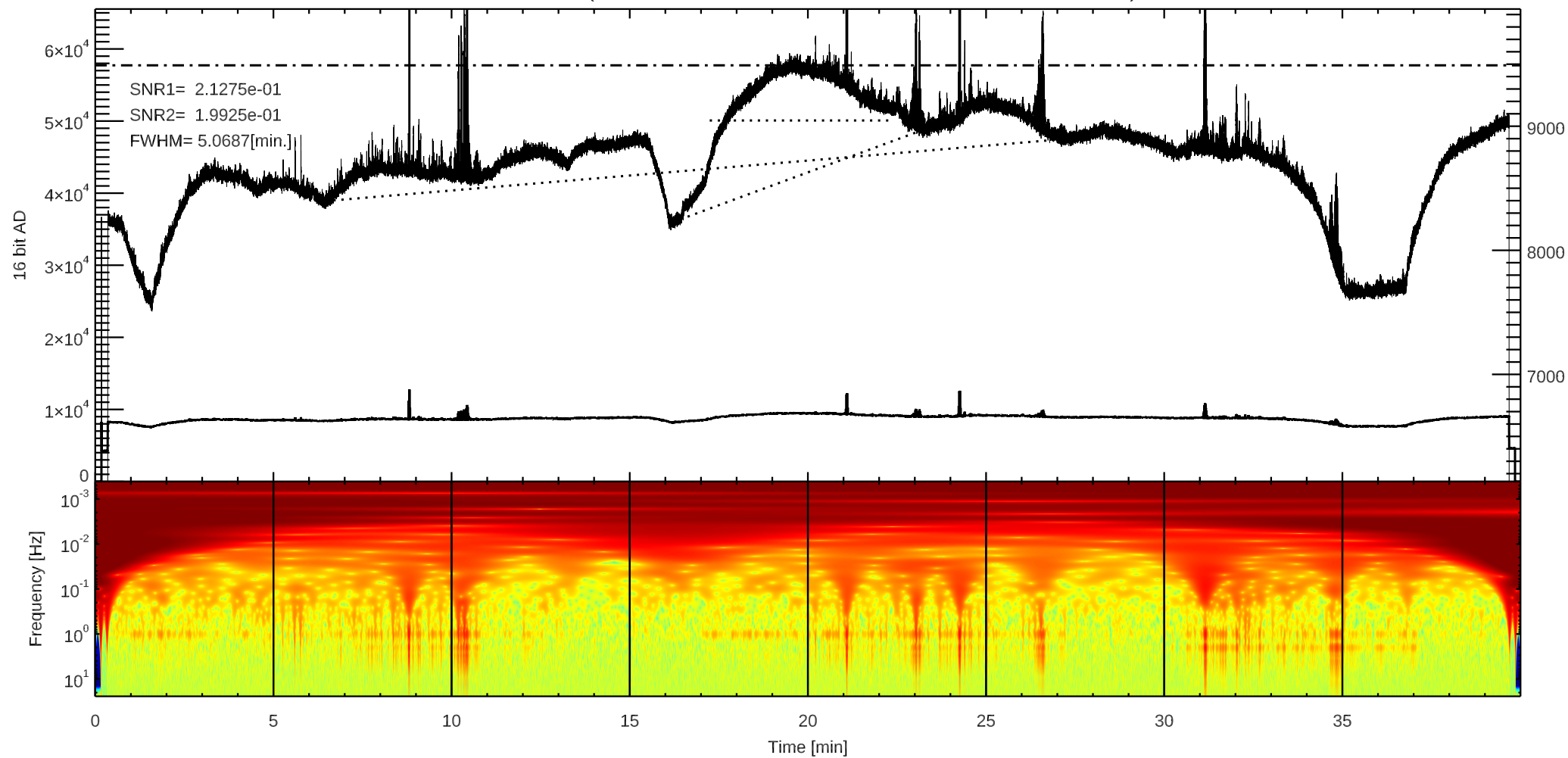
C 3C10 (/home4/archive/swift/dat/2025/12/T20251219180430.dat)
