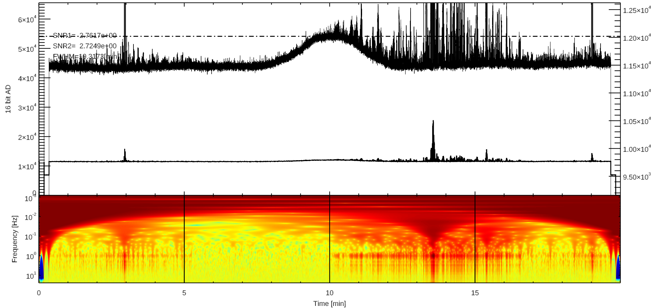
C 3C123 (/home4/archive/fit/dat/2025/12/F20251214224517.dat)
