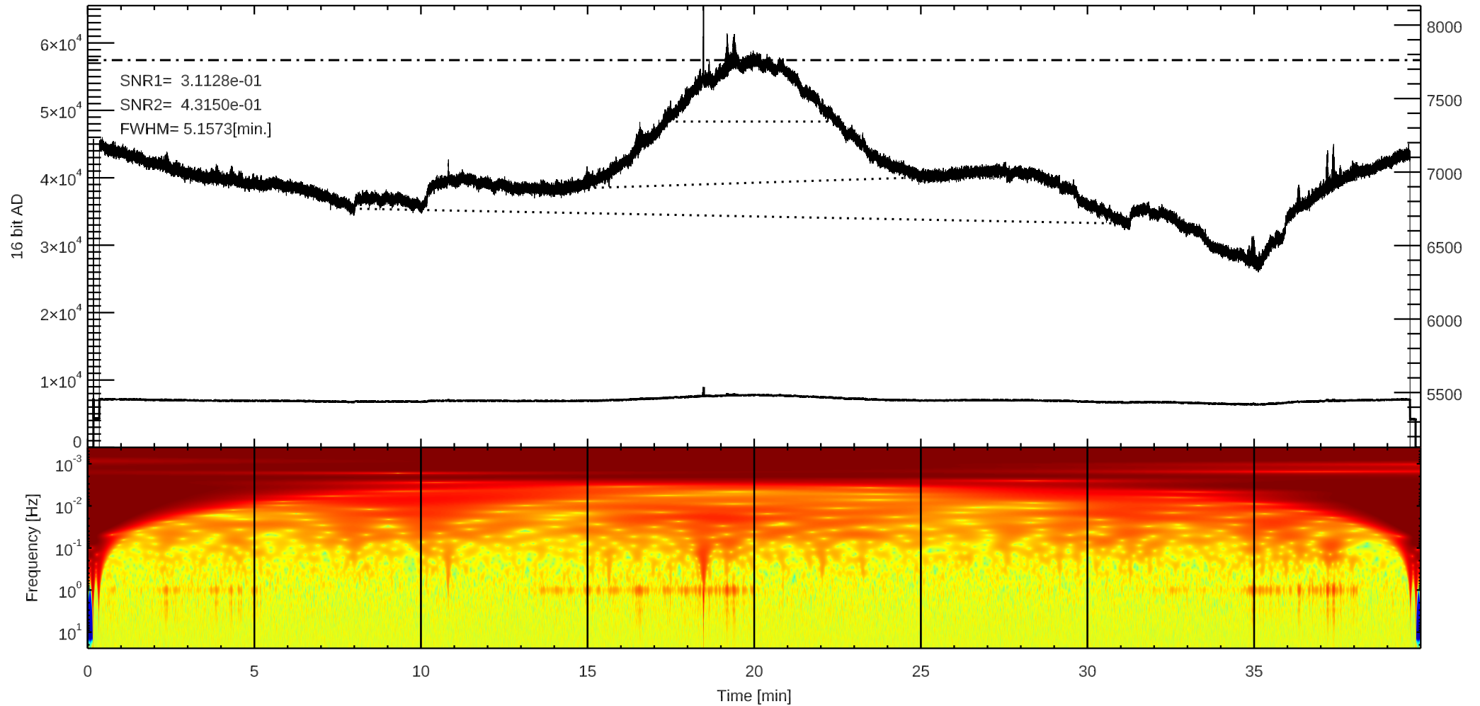
C 3C123 (/home4/archive/swift/dat/2025/12/T20251213223914.dat)
