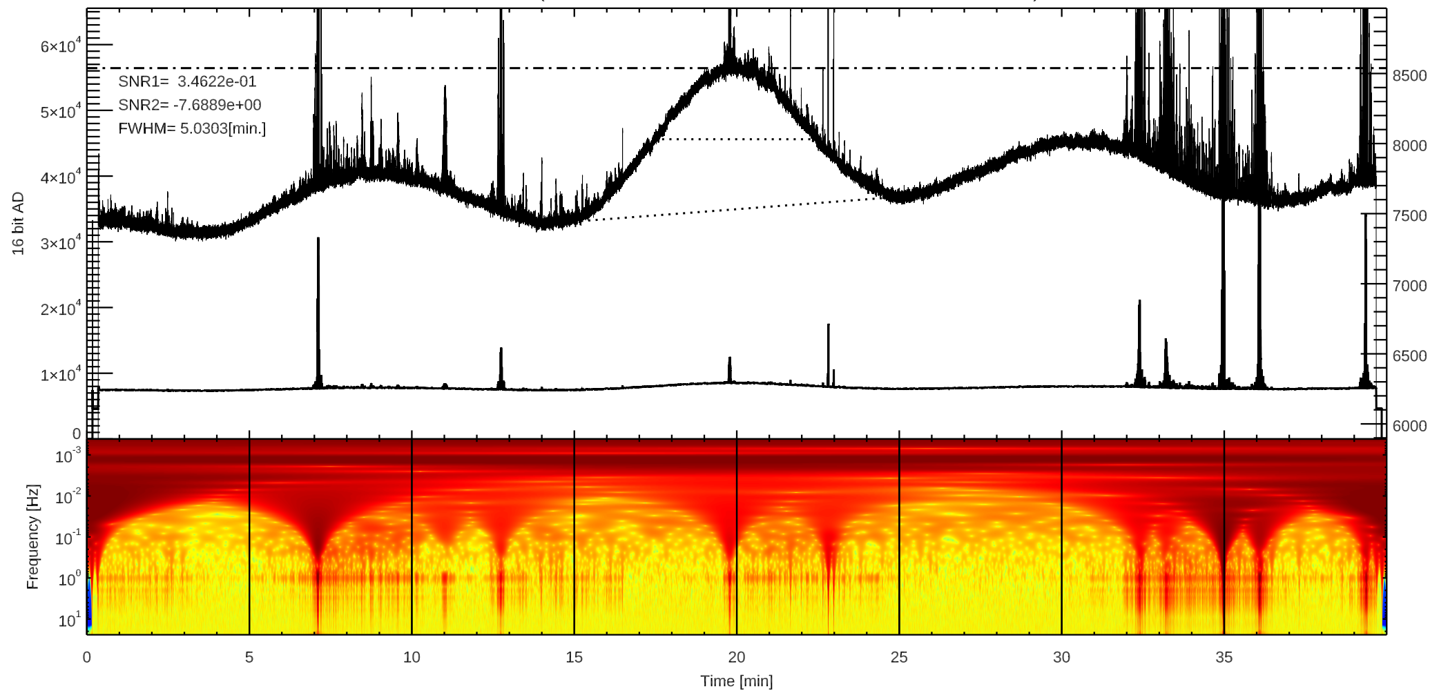
C 3C123 (/home4/archive/swift/dat/2025/12/T20251223215955.dat)
