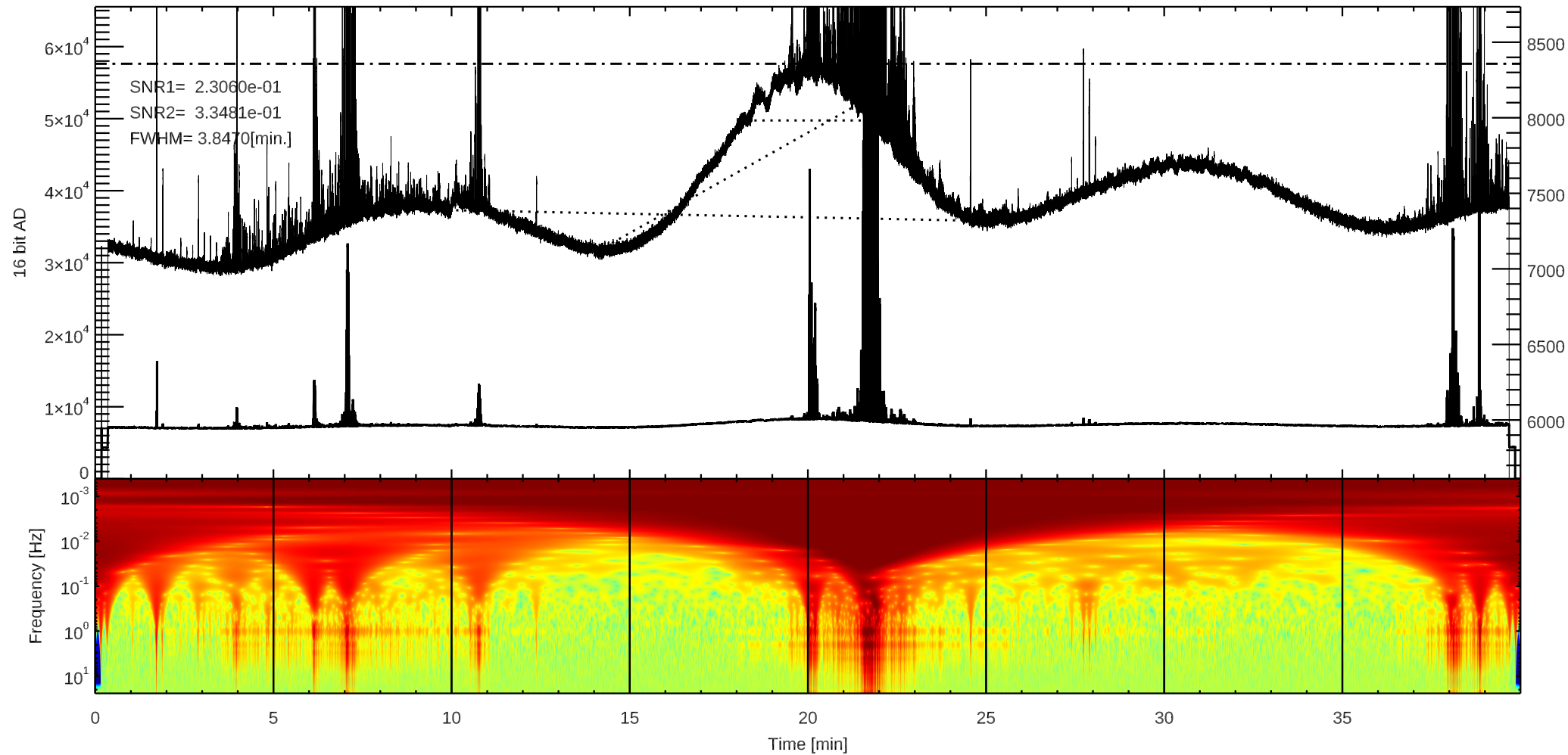
C 3C123 (/home4/archive/swift/dat/2025/12/T20251224215600.dat)
