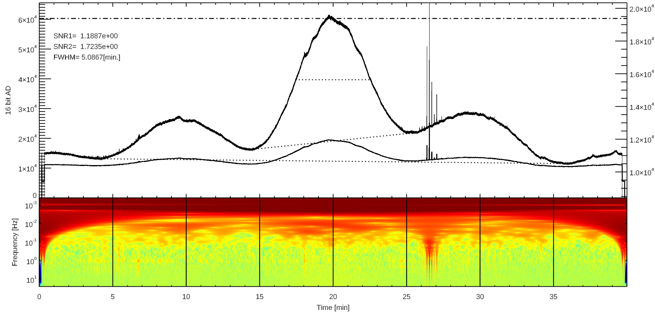
C 3C144 (/home4/archive/swift/dat/2025/12/T20251205001150.dat)
