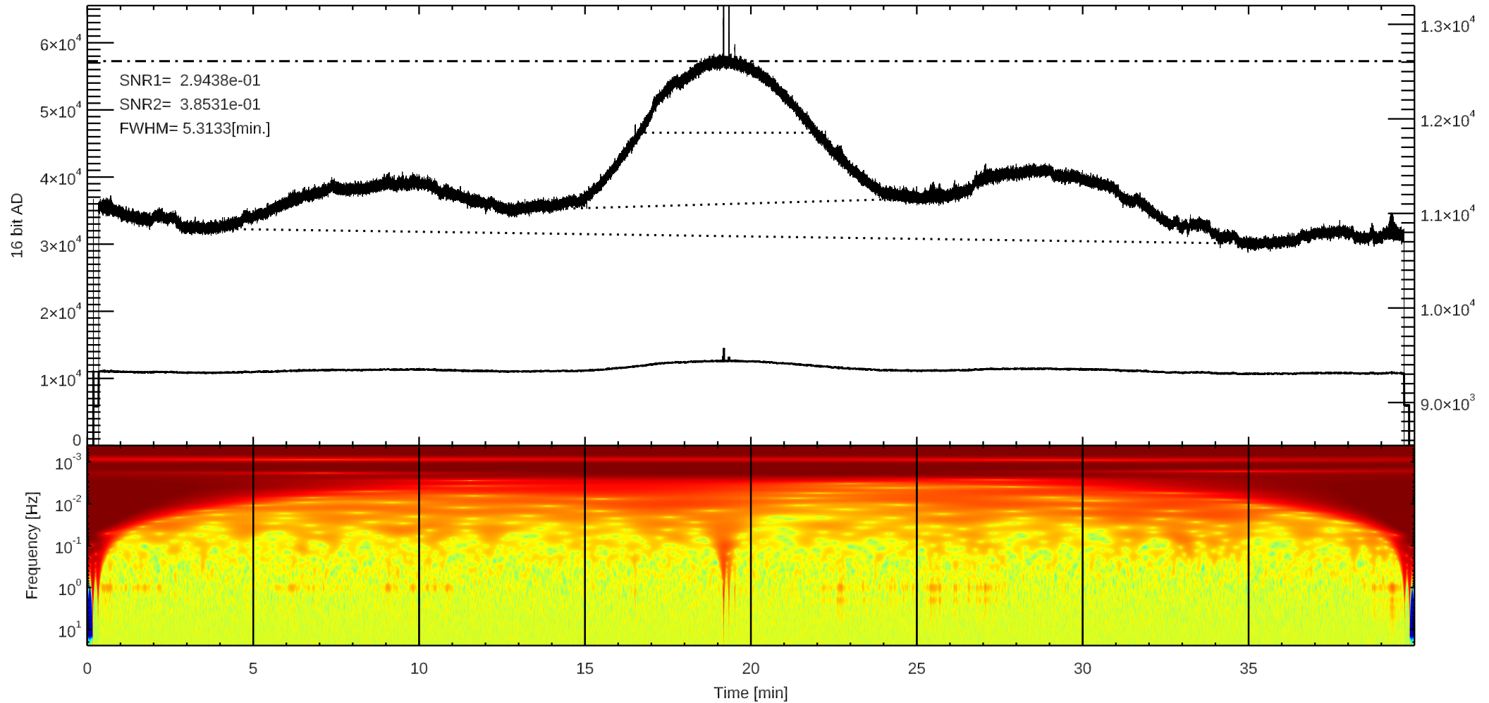
C 3C157 (/home4/archive/swift/dat/2025/12/T20251207004722.dat)
