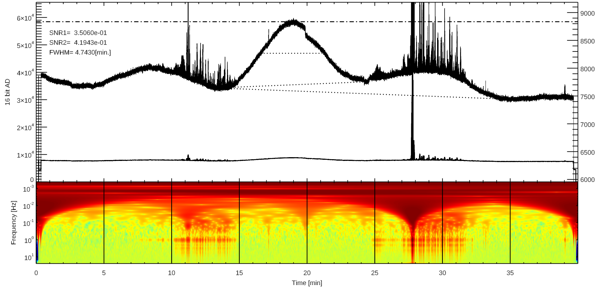
C 3C157 (/home4/archive/swift/dat/2025/12/T20251212002743.dat)
