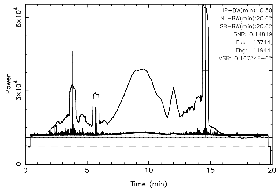
FUJI 3C157 2025/11/30(334)01:24:51-01:44:52JST
