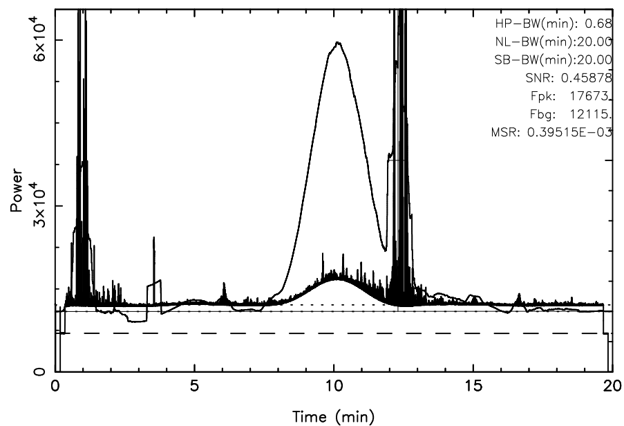
FUJI 3C144 2025/11/30(334)00:41:27-01:01:27JST
