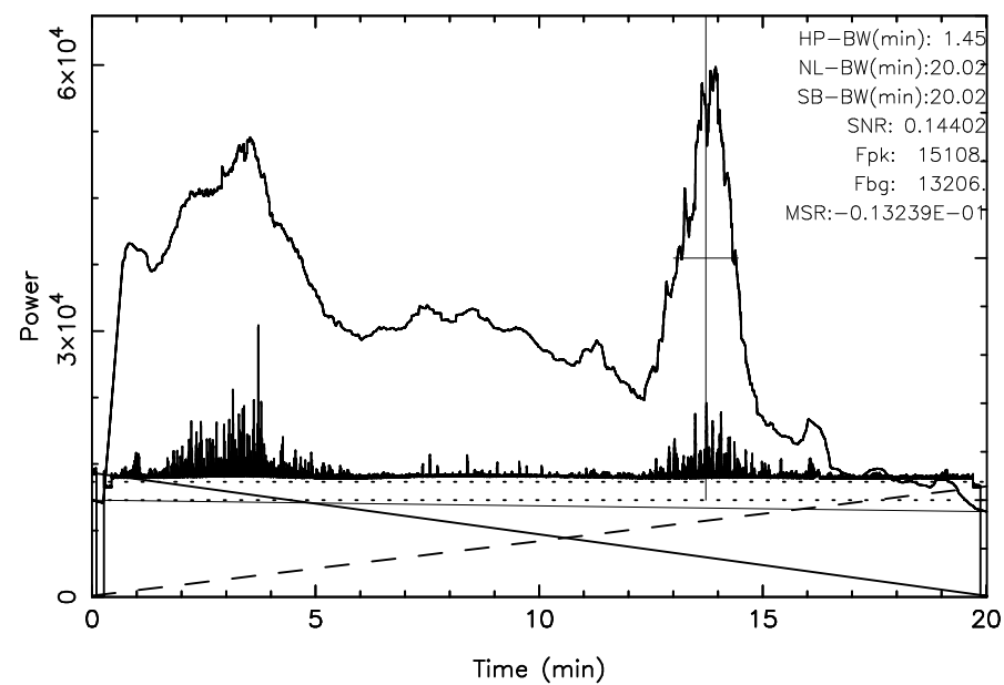
KISO 3C157 2025/11/30(334)01:24:51-01:44:52JST
