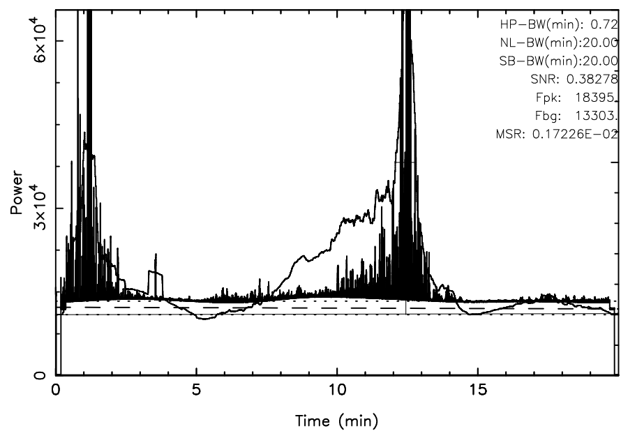
KISO 3C144 2025/11/30(334)00:41:27-01:01:27JST
