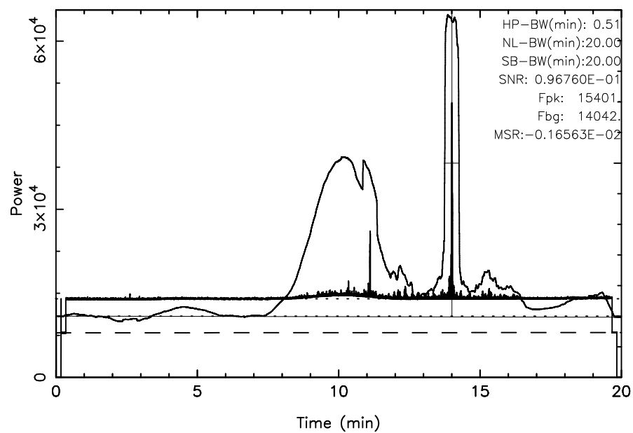
FUJI 3C123 2025/12/06(340)23:16:44-23:36:44JST
