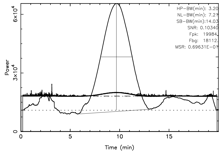
KISO 3C144 2025/12/06(340)00:17:52-00:37:52JST
