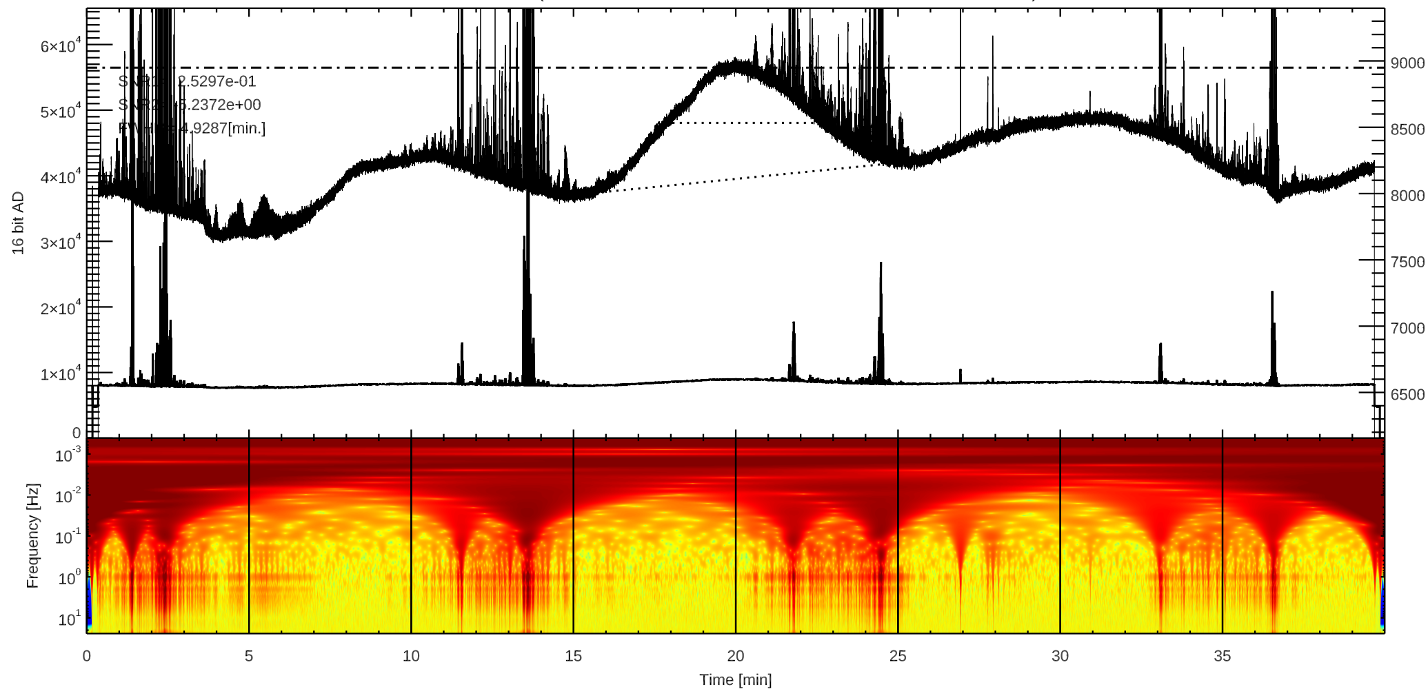
C 3C123 (/home4/archive/swift/dat/2026/01/T20260105210849.dat)
