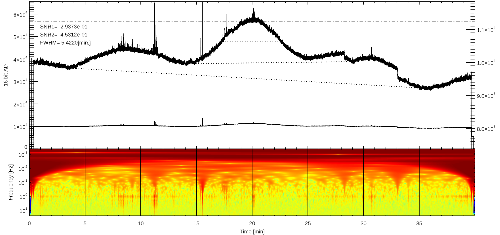
C 3C123 (/home4/archive/swift/dat/2026/01/T20260108205701.dat)
