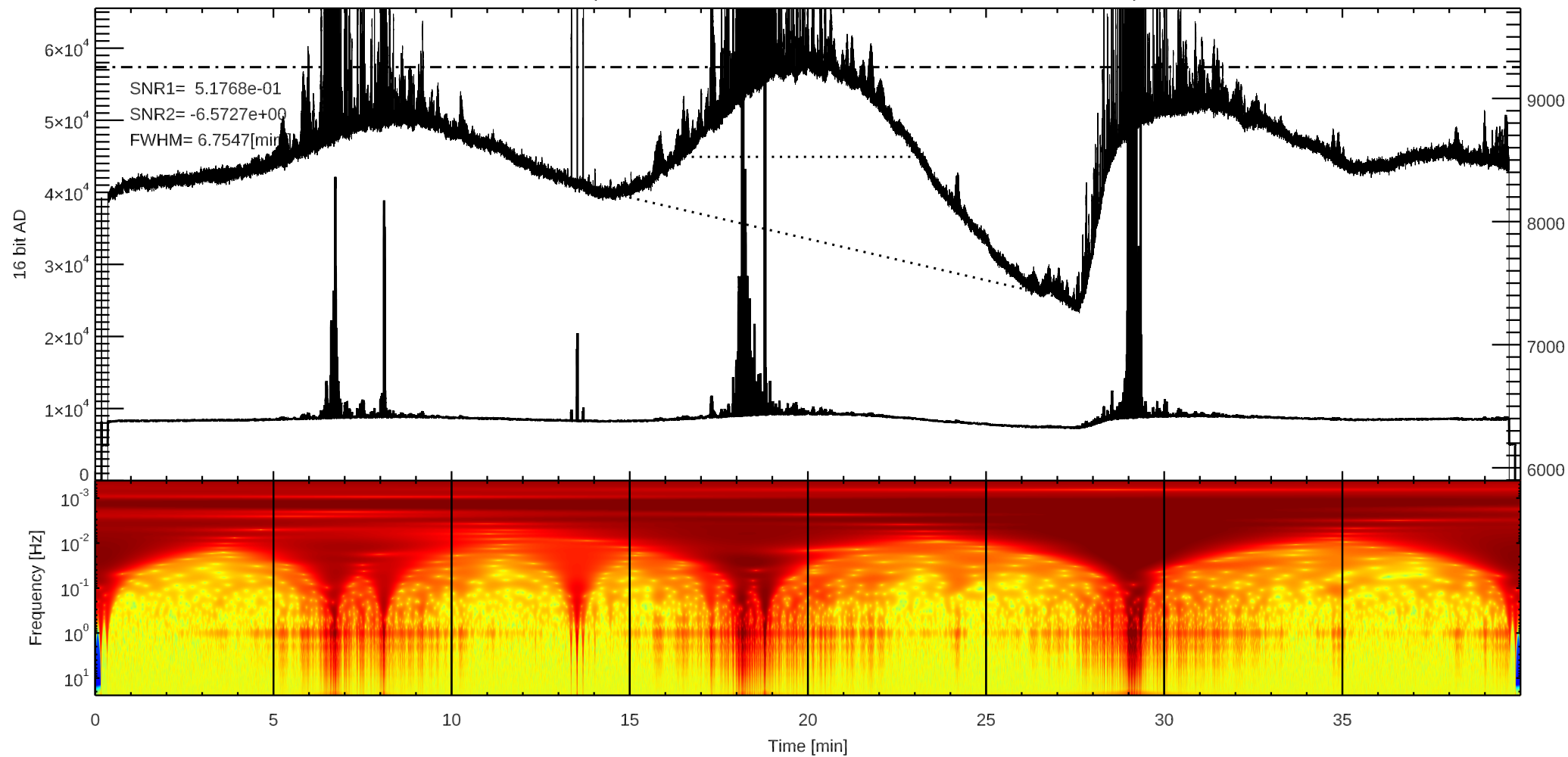
C 3C123 (/home4/archive/swift/dat/2026/01/T20260113203722.dat)
