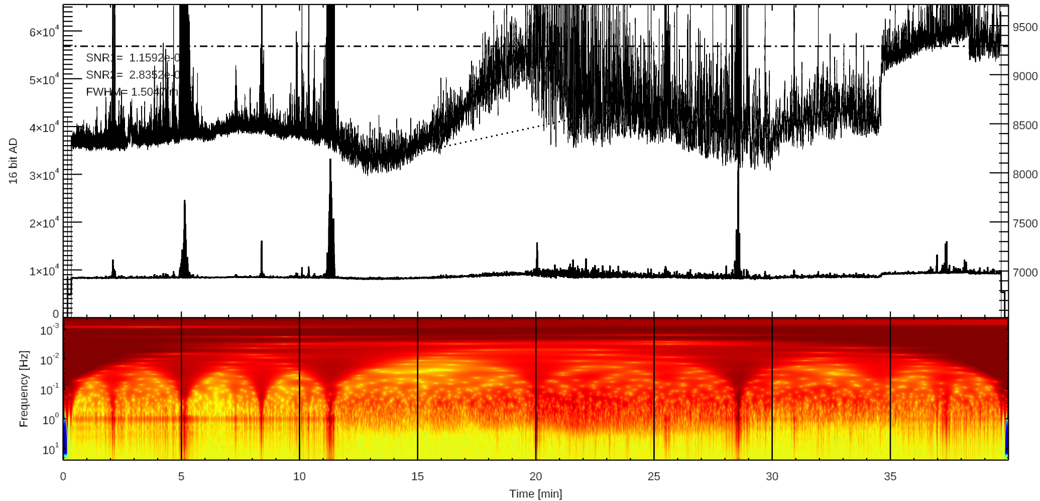
C 3C123 (/home4/archive/swift/dat/2026/01/T20260120200950.dat)
