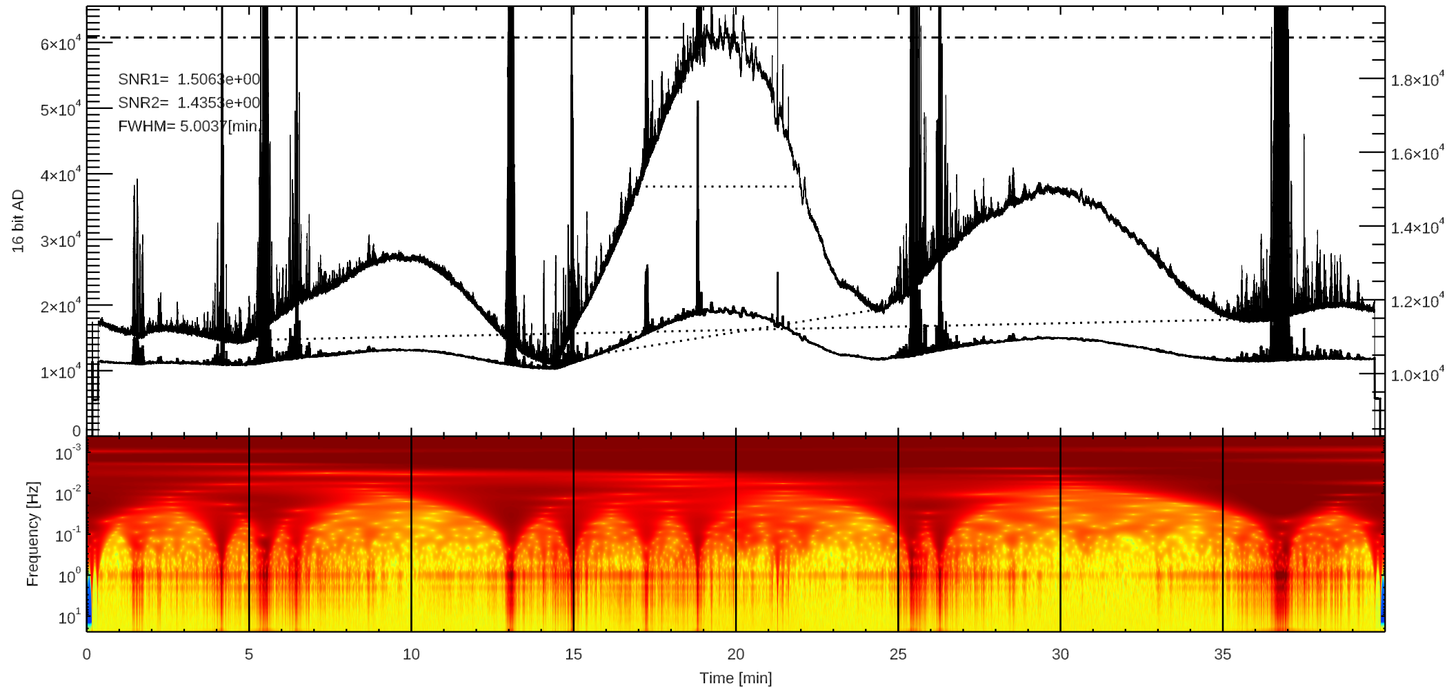
C 3C144 (/home4/archive/swift/dat/2026/01/T20260109215017.dat)
