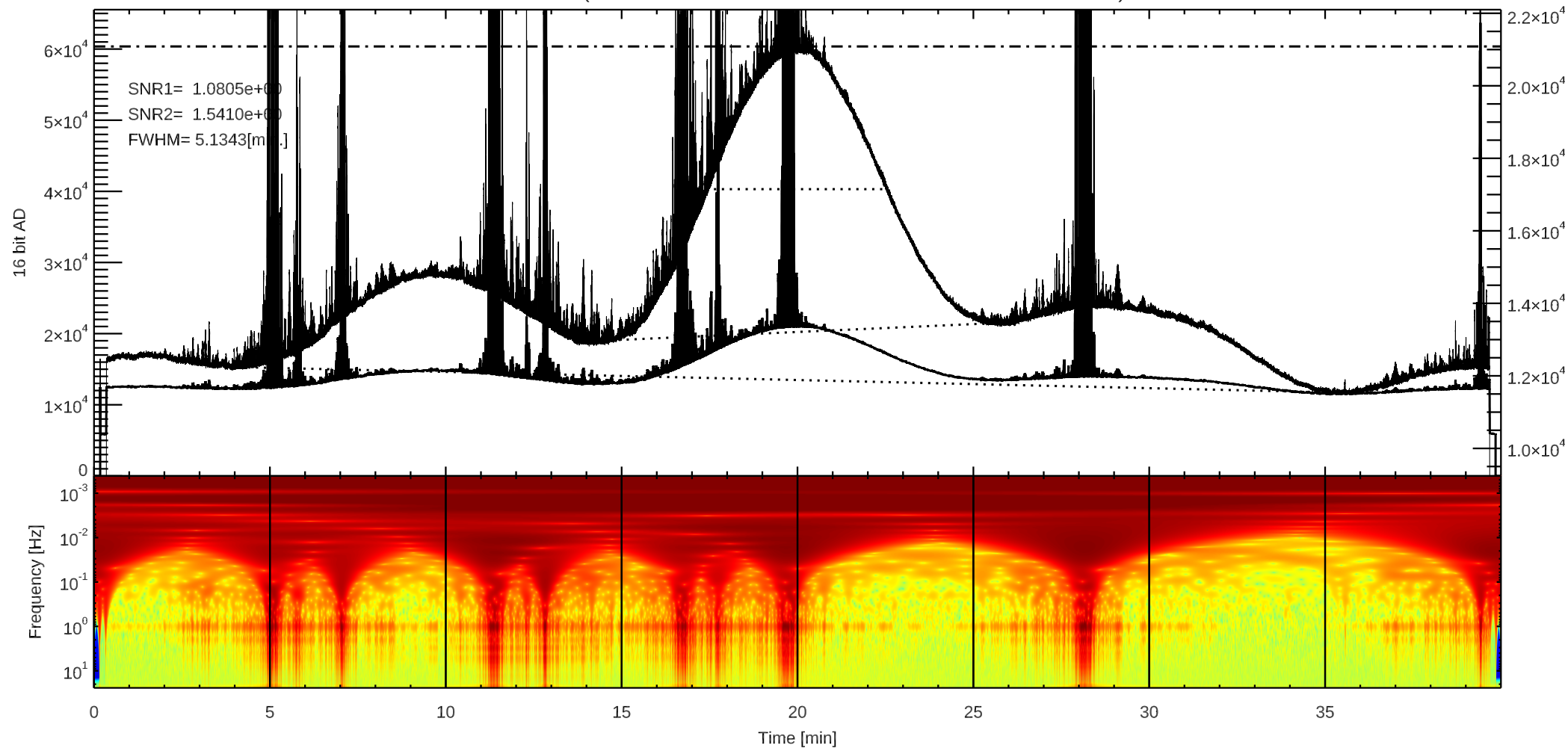
C 3C144 (/home4/archive/swift/dat/2026/01/T20260114213038.dat)
